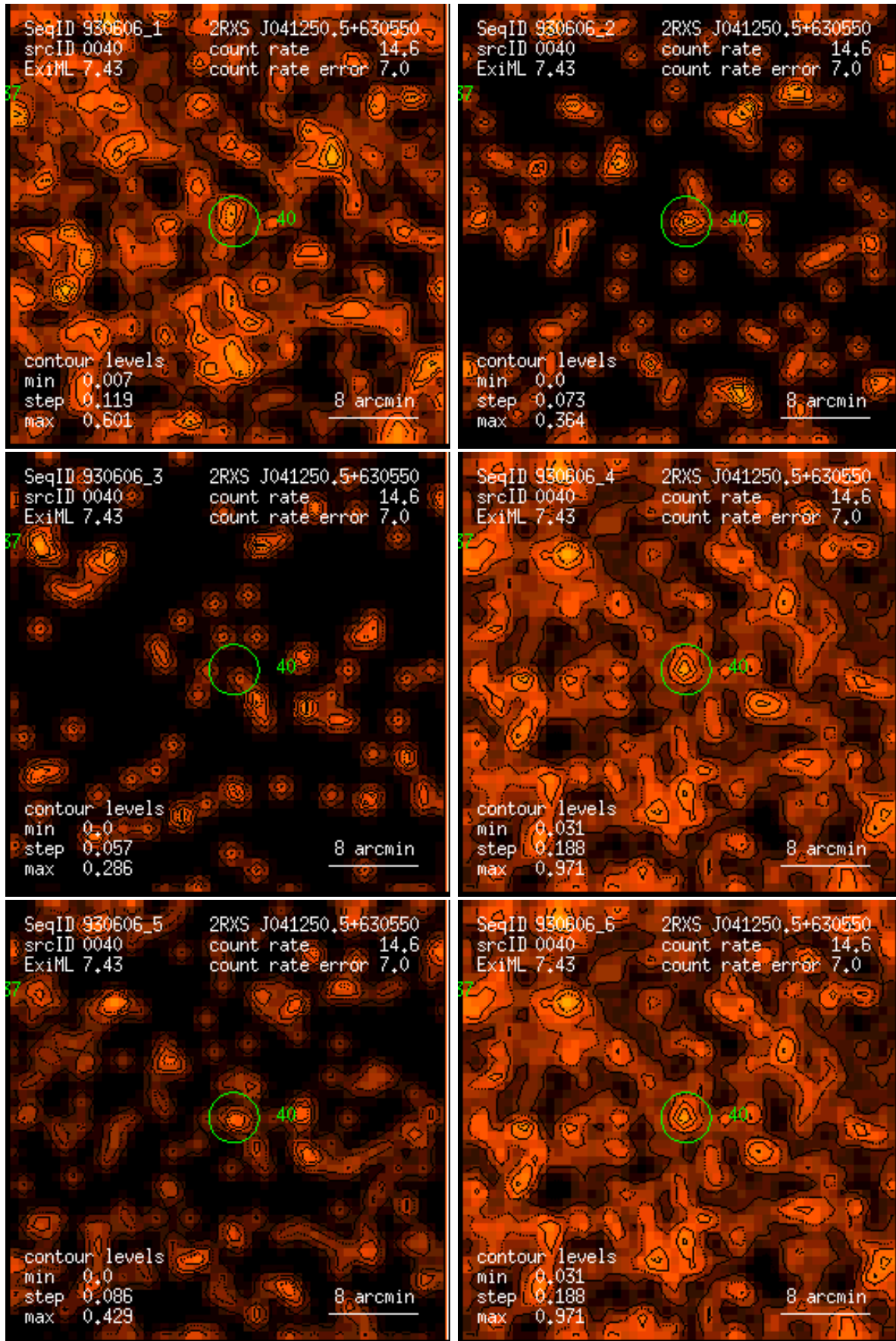
Figure 40: RASS 930606: detection 0040: band rate images, Gaussian filter: (1) PSPC channels 11 – 41, (2) 52 – 90, (3) 91 – 201, (4) 11 – 235, (5) 52 – 201, (6) 11 – 201. Broad band rates in counts/ks. Band rate contour levels in counts/ks/arcmin 2 .
