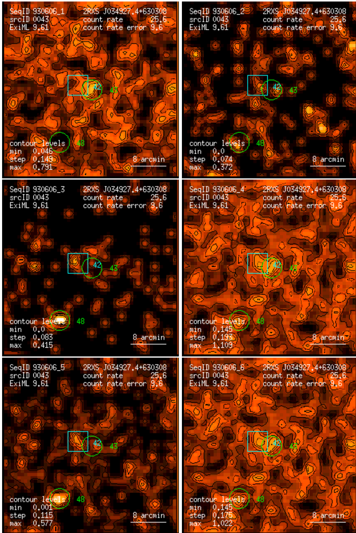
Figure 43: RASS 930606: detection 0043: band rate images, Gaussian filter: (1) PSPC channels 11 – 41, (2) 52 – 90, (3) 91 – 201, (4) 11 – 235, (5) 52 – 201, (6) 11 – 201. Broad band rates in counts/ks. Band rate contour levels in counts/ks/arcmin 2 .
