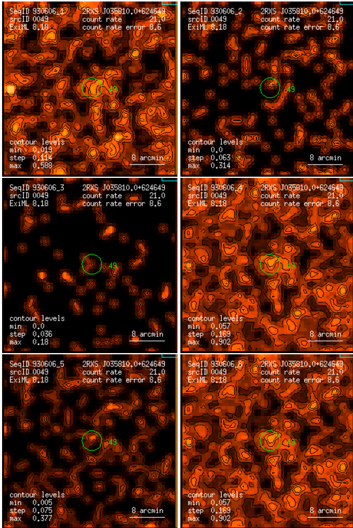
Figure 49: RASS 930606: detection 0049: band rate images, Gaussian filter: (1) PSPC channels 11 – 41, (2) 52 – 90, (3) 91 – 201, (4) 11 – 235, (5) 52 – 201, (6) 11 – 201. Broad band rates in counts/ks. Band rate contour levels in counts/ks/arcmin 2 .
