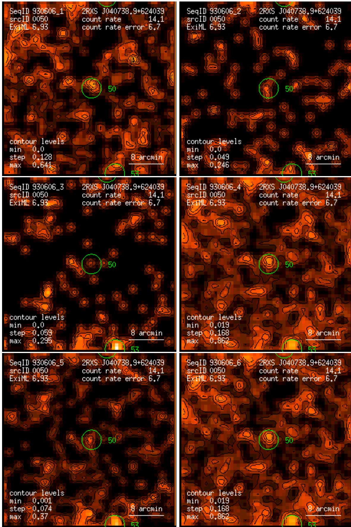
Figure 50: RASS 930606: detection 0050: band rate images, Gaussian filter: (1) PSPC channels 11 – 41, (2) 52 – 90, (3) 91 – 201, (4) 11 – 235, (5) 52 – 201, (6) 11 – 201. Broad band rates in counts/ks. Band rate contour levels in counts/ks/arcmin 2 .
