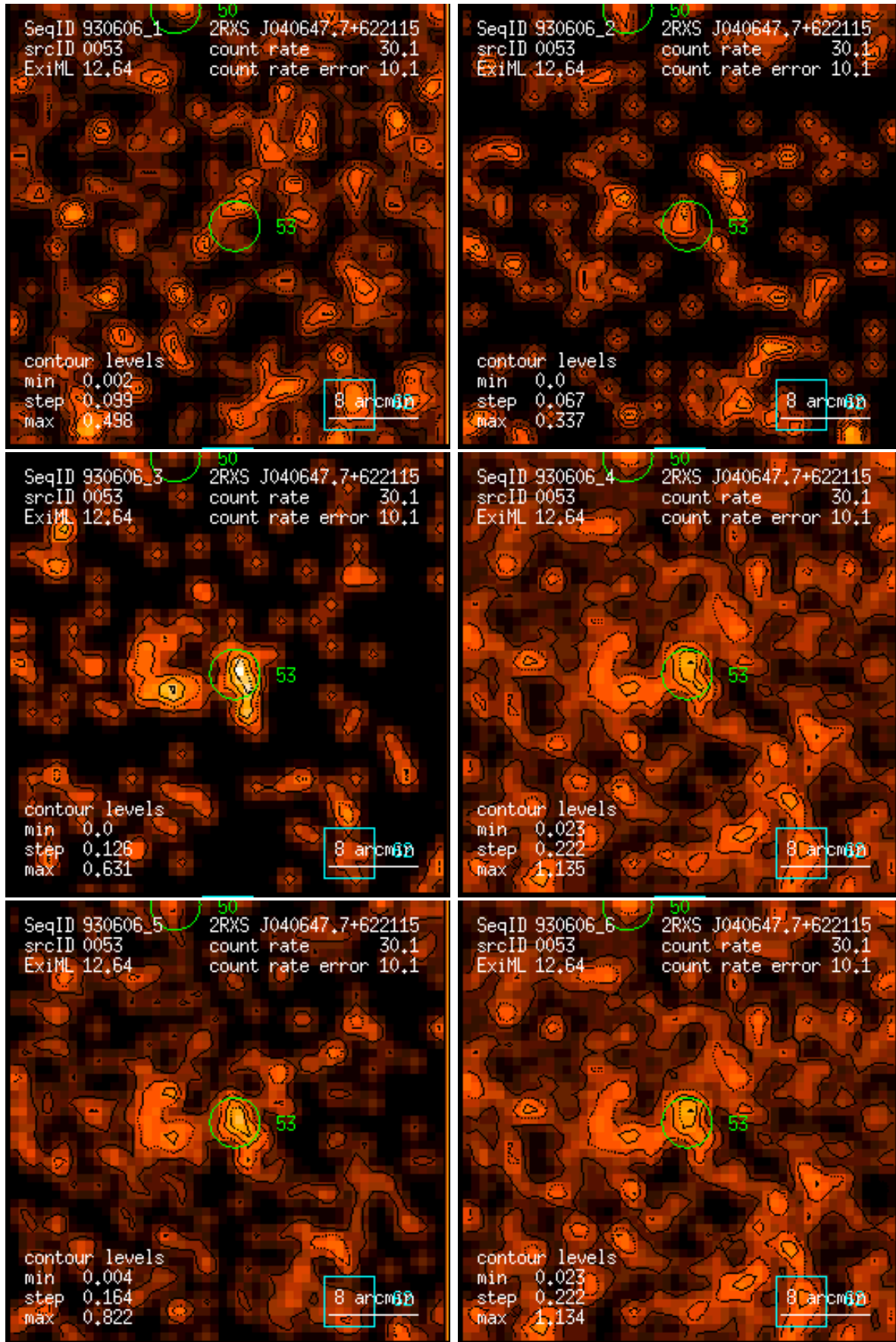
Figure 53: RASS 930606: detection 0053: band rate images, Gaussian filter: (1) PSPC channels 11 – 41, (2) 52 – 90, (3) 91 – 201, (4) 11 – 235, (5) 52 – 201, (6) 11 – 201. Broad band rates in counts/ks. Band rate contour levels in counts/ks/arcmin 2 .
