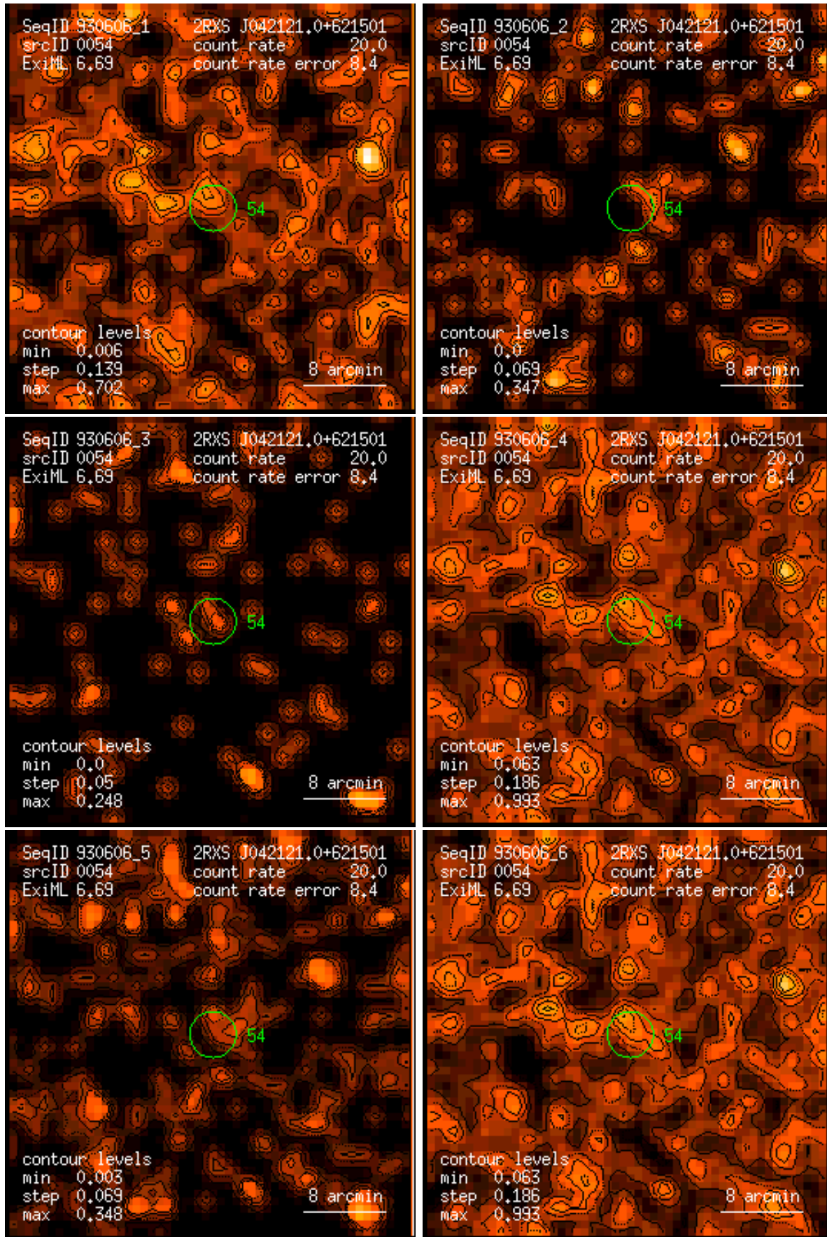
Figure 54: RASS 930606: detection 0054: band rate images, Gaussian filter: (1) PSPC channels 11 – 41, (2) 52 – 90, (3) 91 – 201, (4) 11 – 235, (5) 52 – 201, (6) 11 – 201. Broad band rates in counts/ks. Band rate contour levels in counts/ks/arcmin 2 .
