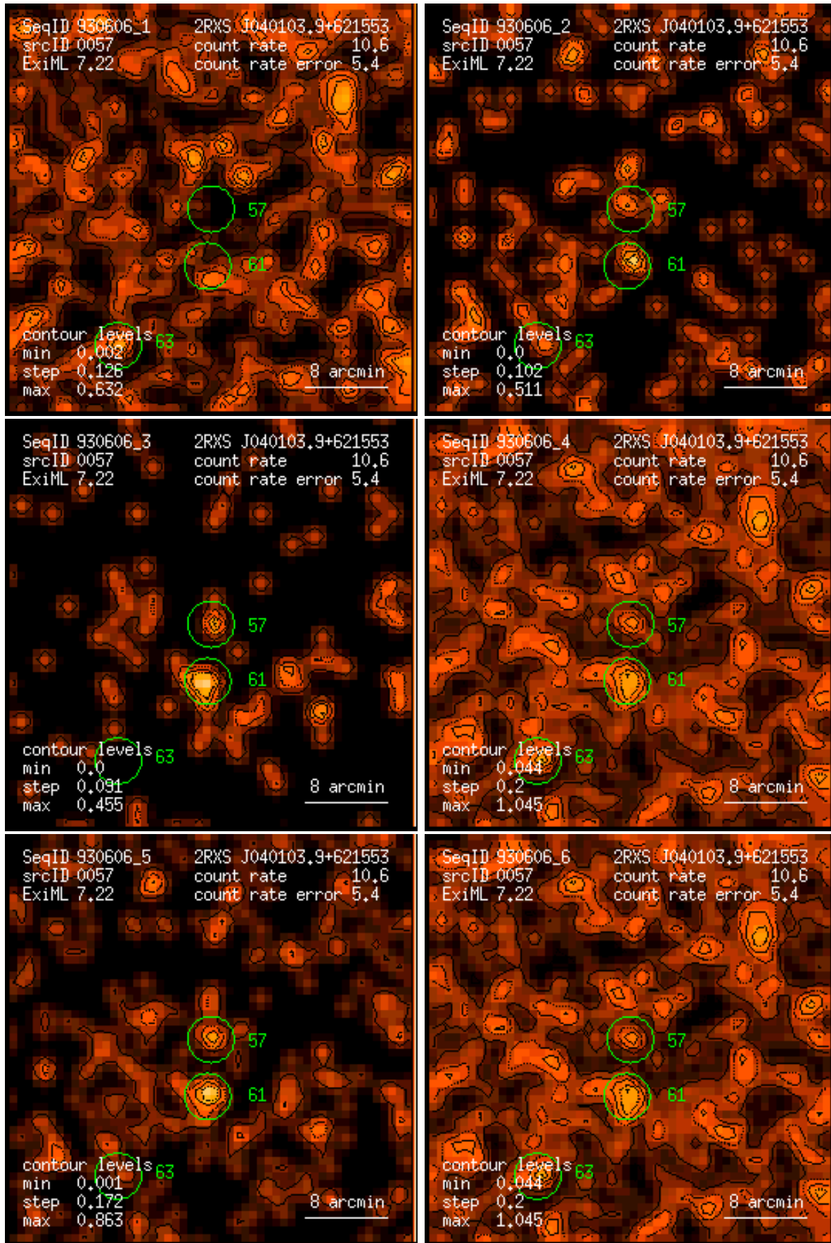
Figure 57: RASS 930606: detection 0057: band rate images, Gaussian filter: (1) PSPC channels 11 – 41, (2) 52 – 90, (3) 91 – 201, (4) 11 – 235, (5) 52 – 201, (6) 11 – 201. Broad band rates in counts/ks. Band rate contour levels in counts/ks/arcmin 2 .
