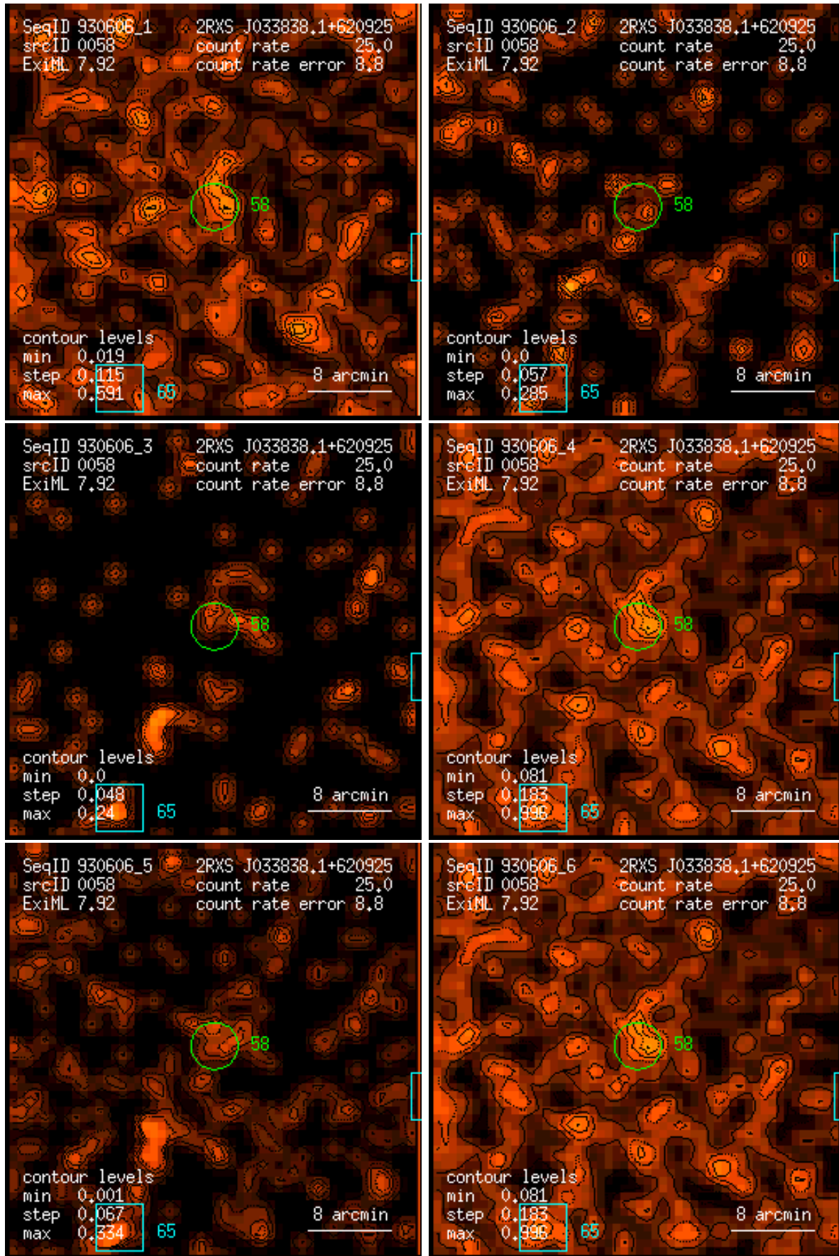
Figure 58: RASS 930606: detection 0058: band rate images, Gaussian filter: (1) PSPC channels 11 – 41, (2) 52 – 90, (3) 91 – 201, (4) 11 – 235, (5) 52 – 201, (6) 11 – 201. Broad band rates in counts/ks. Band rate contour levels in counts/ks/arcmin 2 .
