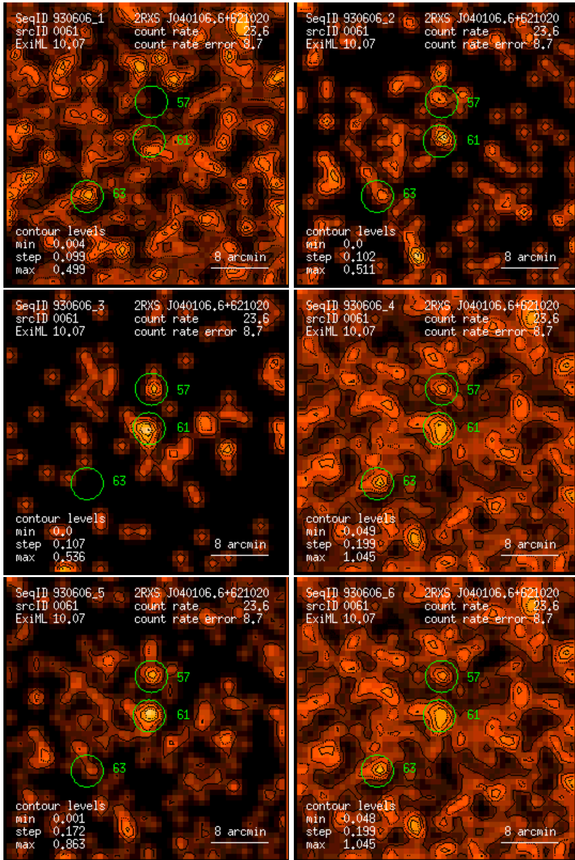
Figure 61: RASS 930606: detection 0061: band rate images, Gaussian filter: (1) PSPC channels 11 – 41, (2) 52 – 90, (3) 91 – 201, (4) 11 – 235, (5) 52 – 201, (6) 11 – 201. Broad band rates in counts/ks. Band rate contour levels in counts/ks/arcmin 2 .
