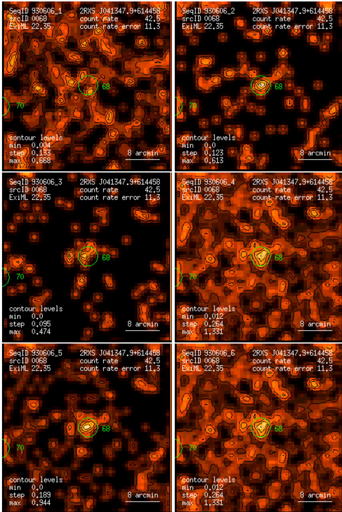
Figure 68: RASS 930606: detection 0068: band rate images, Gaussian filter: (1) PSPC channels 11 – 41, (2) 52 – 90, (3) 91 – 201, (4) 11 – 235, (5) 52 – 201, (6) 11 – 201. Broad band rates in counts/ks. Band rate contour levels in counts/ks/arcmin 2 .
