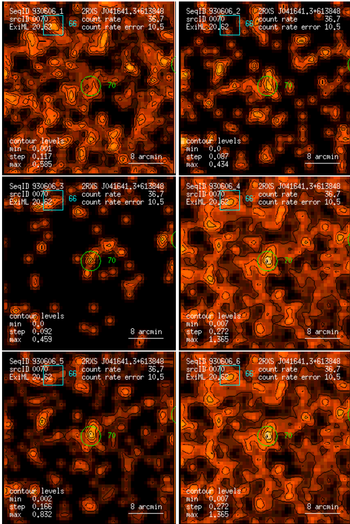
Figure 70: RASS 930606: detection 0070: band rate images, Gaussian filter: (1) PSPC channels 11 – 41, (2) 52 – 90, (3) 91 – 201, (4) 11 – 235, (5) 52 – 201, (6) 11 – 201. Broad band rates in counts/ks. Band rate contour levels in counts/ks/arcmin 2 .
