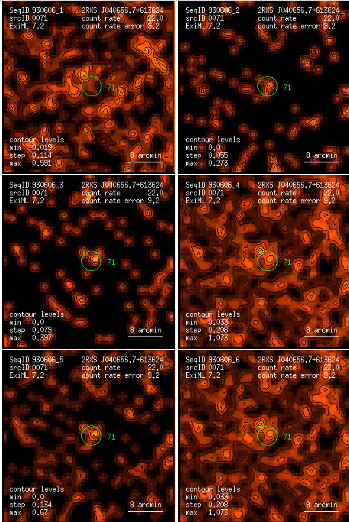
Figure 71: RASS 930606: detection 0071: band rate images, Gaussian filter: (1) PSPC channels 11 – 41, (2) 52 – 90, (3) 91 – 201, (4) 11 – 235, (5) 52 – 201, (6) 11 – 201. Broad band rates in counts/ks. Band rate contour levels in counts/ks/arcmin 2 .
