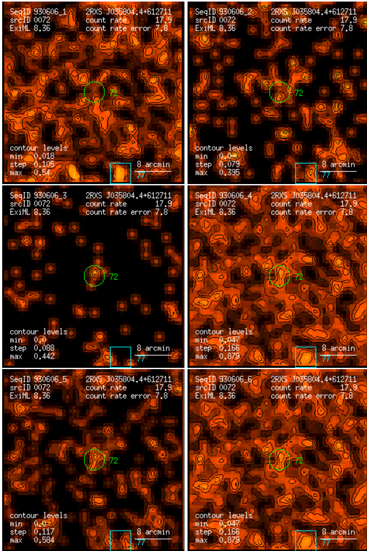
Figure 72: RASS 930606: detection 0072: band rate images, Gaussian filter: (1) PSPC channels 11 – 41, (2) 52 – 90, (3) 91 – 201, (4) 11 – 235, (5) 52 – 201, (6) 11 – 201. Broad band rates in counts/ks. Band rate contour levels in counts/ks/arcmin 2 .
