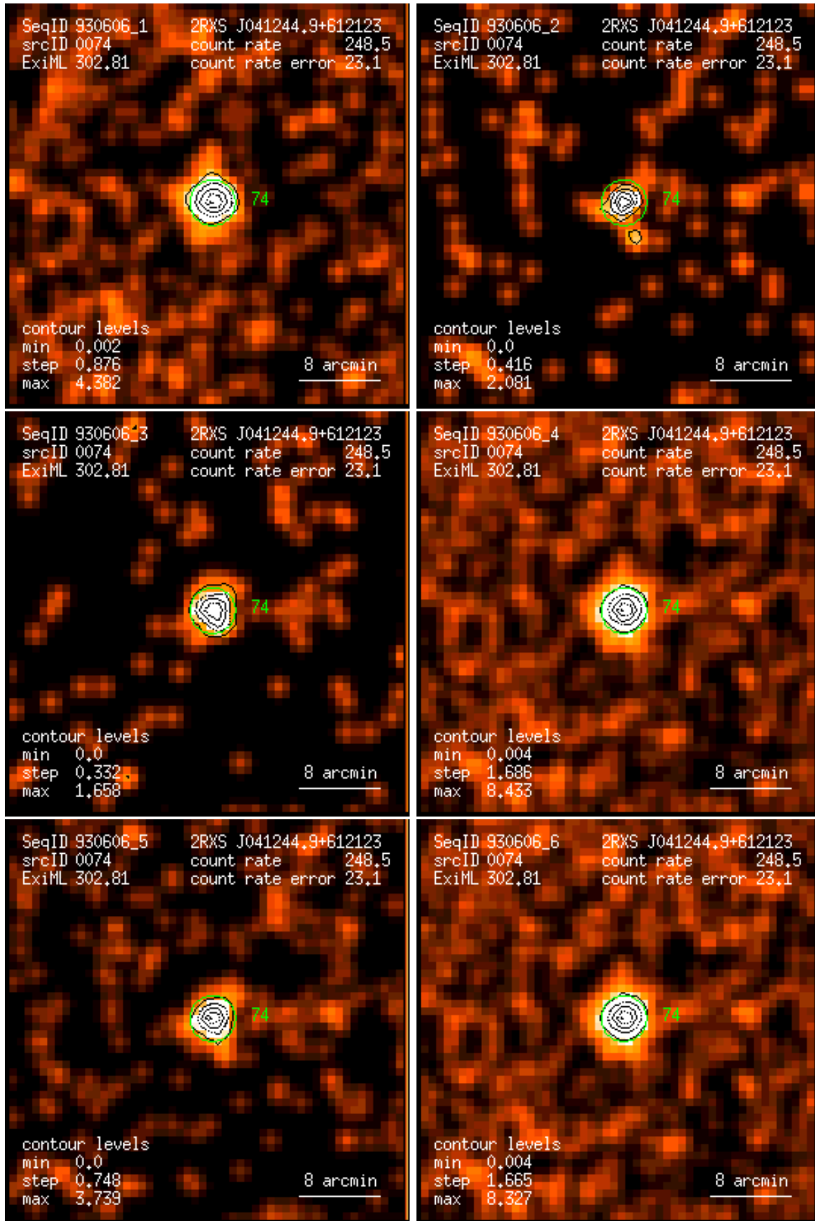
Figure 74: RASS 930606: detection 0074: band rate images, Gaussian filter: (1) PSPC channels 11 – 41, (2) 52 – 90, (3) 91 – 201, (4) 11 – 235, (5) 52 – 201, (6) 11 – 201. Broad band rates in counts/ks. Band rate contour levels in counts/ks/arcmin 2 .
