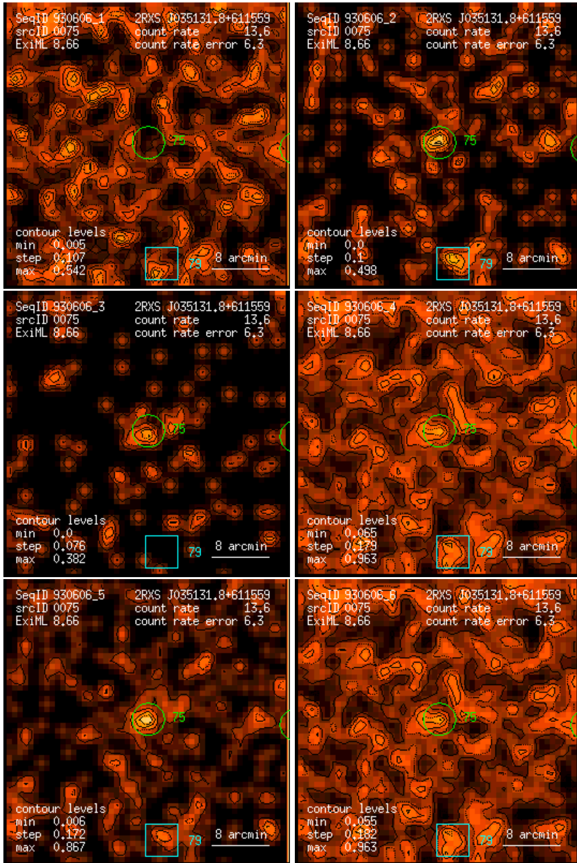
Figure 75: RASS 930606: detection 0075: band rate images, Gaussian filter: (1) PSPC channels 11 – 41, (2) 52 – 90, (3) 91 – 201, (4) 11 – 235, (5) 52 – 201, (6) 11 – 201. Broad band rates in counts/ks. Band rate contour levels in counts/ks/arcmin 2 .
