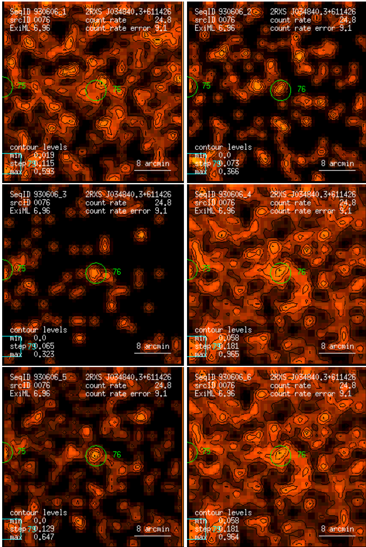
Figure 76: RASS 930606: detection 0076: band rate images, Gaussian filter: (1) PSPC channels 11 – 41, (2) 52 – 90, (3) 91 – 201, (4) 11 – 235, (5) 52 – 201, (6) 11 – 201. Broad band rates in counts/ks. Band rate contour levels in counts/ks/arcmin 2 .
