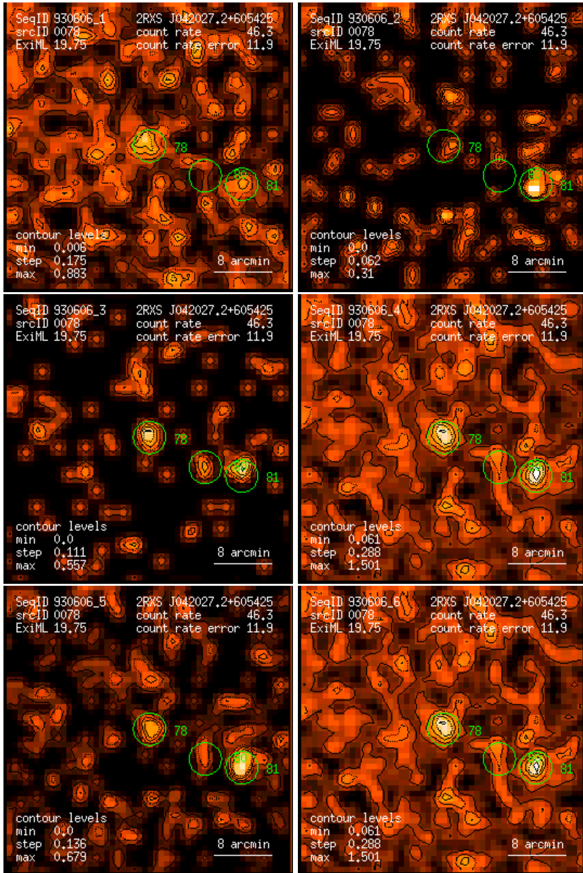
Figure 78: RASS 930606: detection 0078: band rate images, Gaussian filter: (1) PSPC channels 11 – 41, (2) 52 – 90, (3) 91 – 201, (4) 11 – 235, (5) 52 – 201, (6) 11 – 201. Broad band rates in counts/ks. Band rate contour levels in counts/ks/arcmin 2 .
