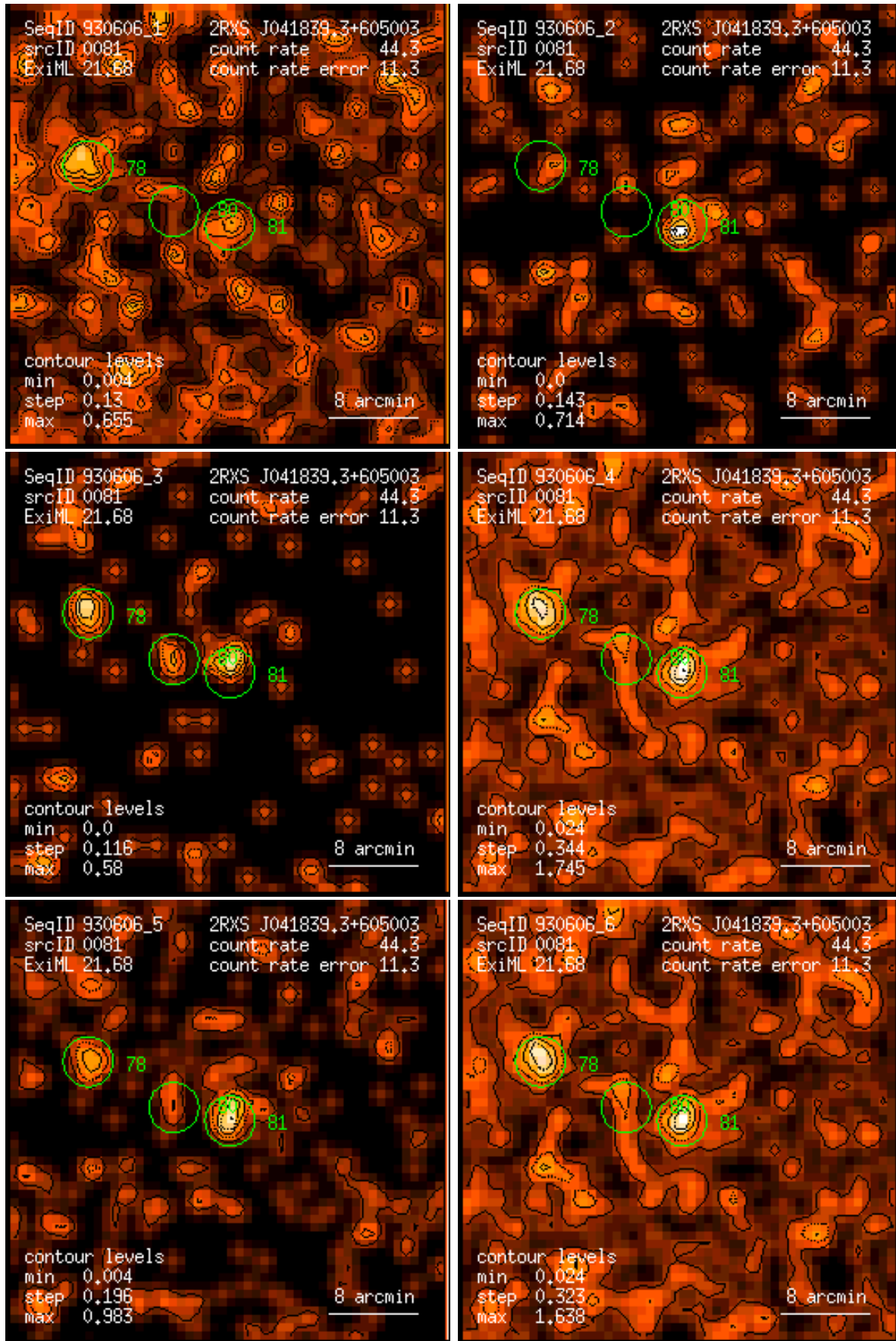
Figure 81: RASS 930606: detection 0081: band rate images, Gaussian filter: (1) PSPC channels 11 – 41, (2) 52 – 90, (3) 91 – 201, (4) 11 – 235, (5) 52 – 201, (6) 11 – 201. Broad band rates in counts/ks. Band rate contour levels in counts/ks/arcmin 2 .
