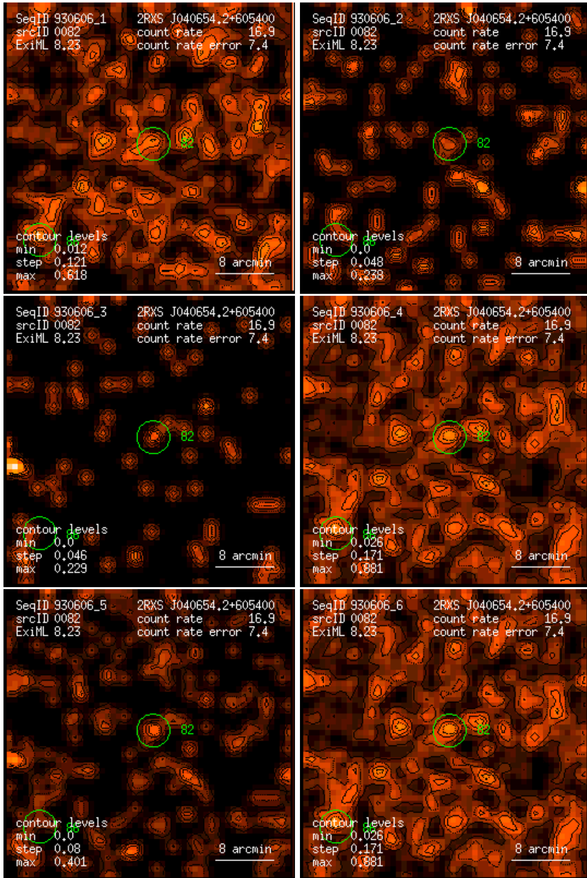
Figure 82: RASS 930606: detection 0082: band rate images, Gaussian filter: (1) PSPC channels 11 – 41, (2) 52 – 90, (3) 91 – 201, (4) 11 – 235, (5) 52 – 201, (6) 11 – 201. Broad band rates in counts/ks. Band rate contour levels in counts/ks/arcmin 2 .
