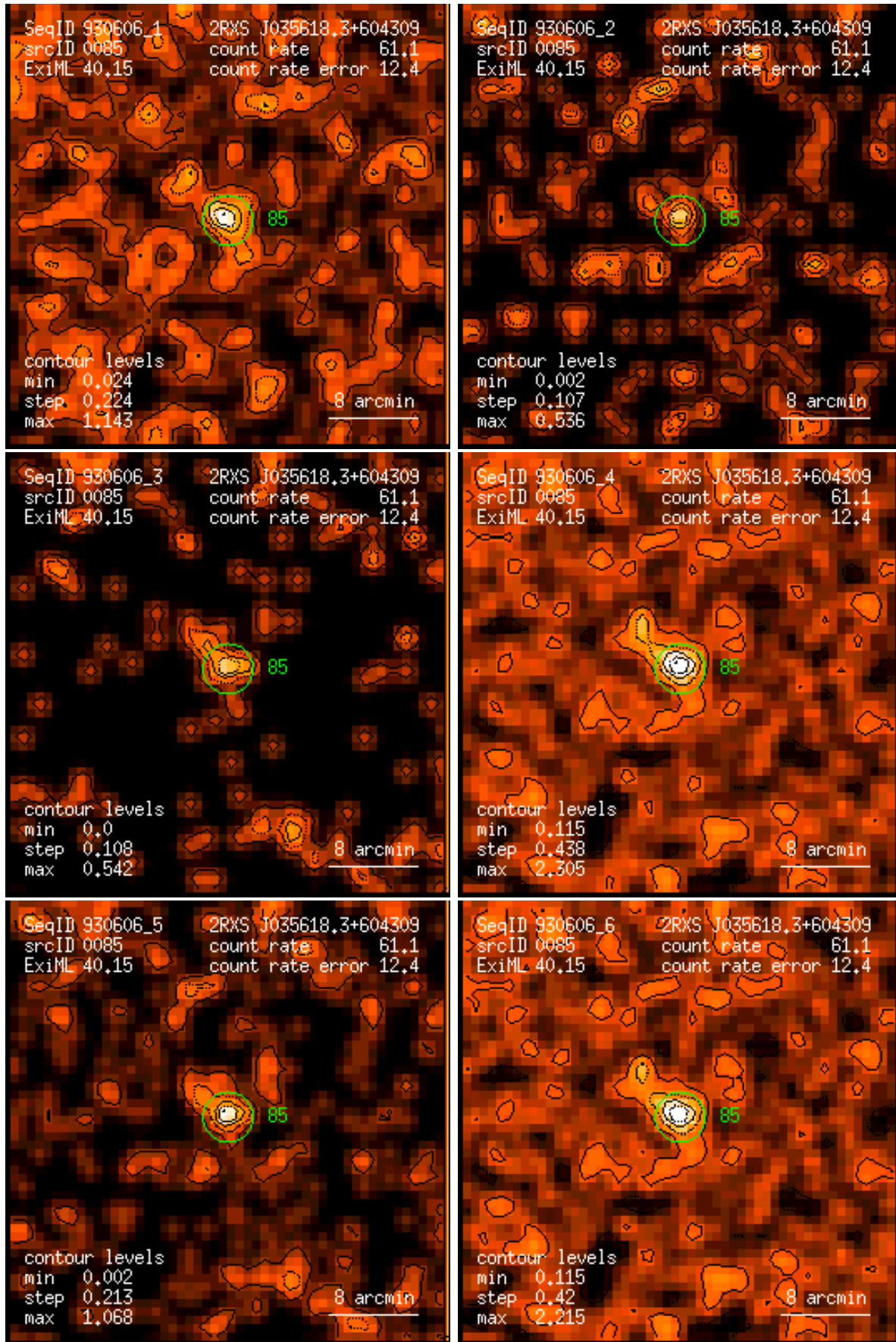
Figure 85: RASS 930606: detection 0085: band rate images, Gaussian filter: (1) PSPC channels 11 – 41, (2) 52 – 90, (3) 91 – 201, (4) 11 – 235, (5) 52 – 201, (6) 11 – 201. Broad band rates in counts/ks. Band rate contour levels in counts/ks/arcmin 2 .
