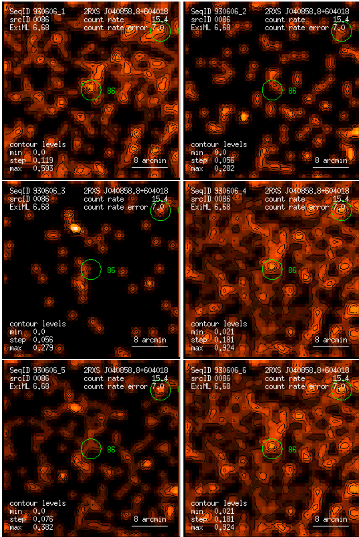
Figure 86: RASS 930606: detection 0086: band rate images, Gaussian filter: (1) PSPC channels 11 – 41, (2) 52 – 90, (3) 91 – 201, (4) 11 – 235, (5) 52 – 201, (6) 11 – 201. Broad band rates in counts/ks. Band rate contour levels in counts/ks/arcmin 2 .
