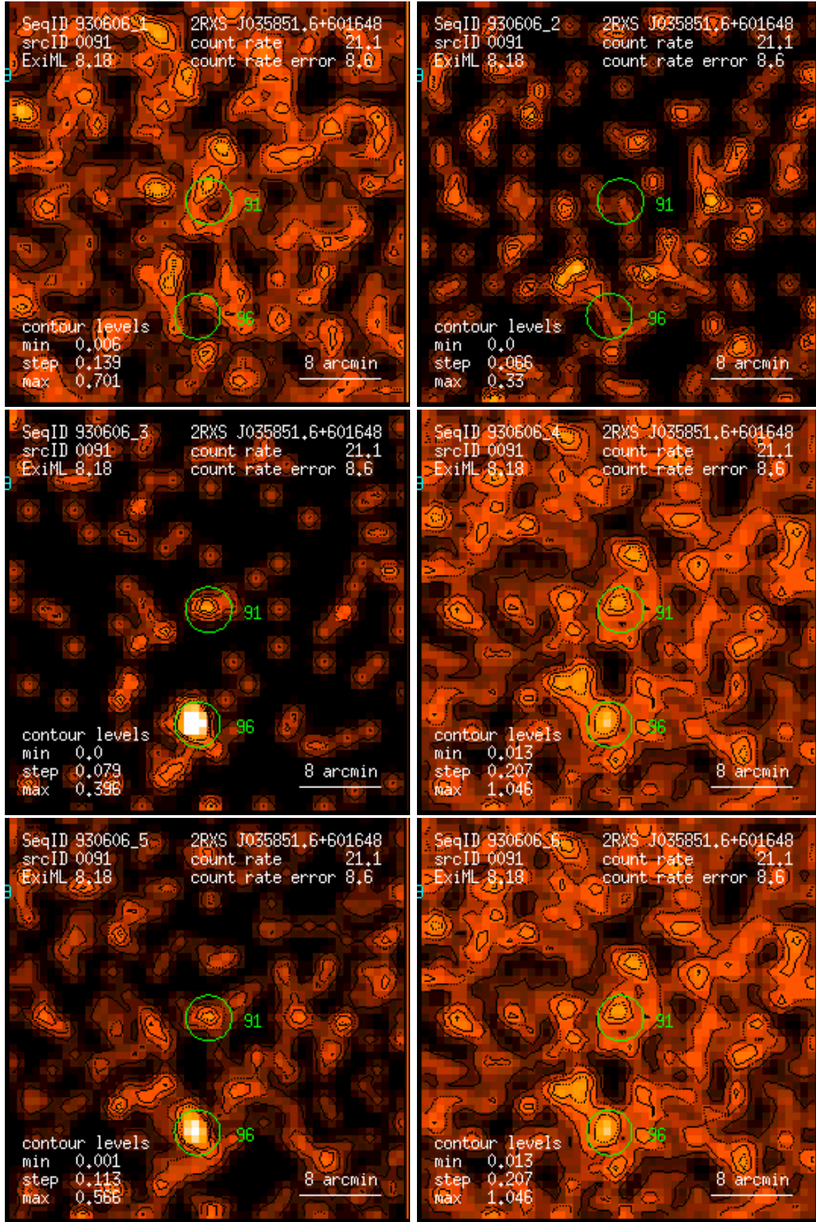
Figure 91: RASS 930606: detection 0091: band rate images, Gaussian filter: (1) PSPC channels 11 – 41, (2) 52 – 90, (3) 91 – 201, (4) 11 – 235, (5) 52 – 201, (6) 11 – 201. Broad band rates in counts/ks. Band rate contour levels in counts/ks/arcmin 2 .
