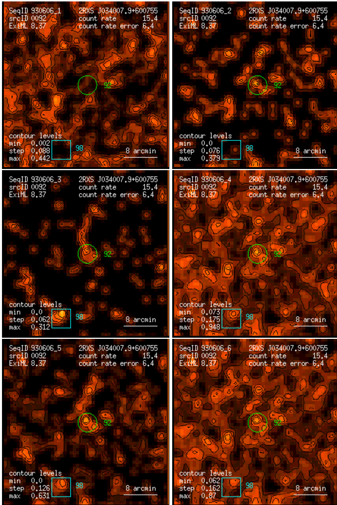
Figure 92: RASS 930606: detection 0092: band rate images, Gaussian filter: (1) PSPC channels 11 – 41, (2) 52 – 90, (3) 91 – 201, (4) 11 – 235, (5) 52 – 201, (6) 11 – 201. Broad band rates in counts/ks. Band rate contour levels in counts/ks/arcmin 2 .
