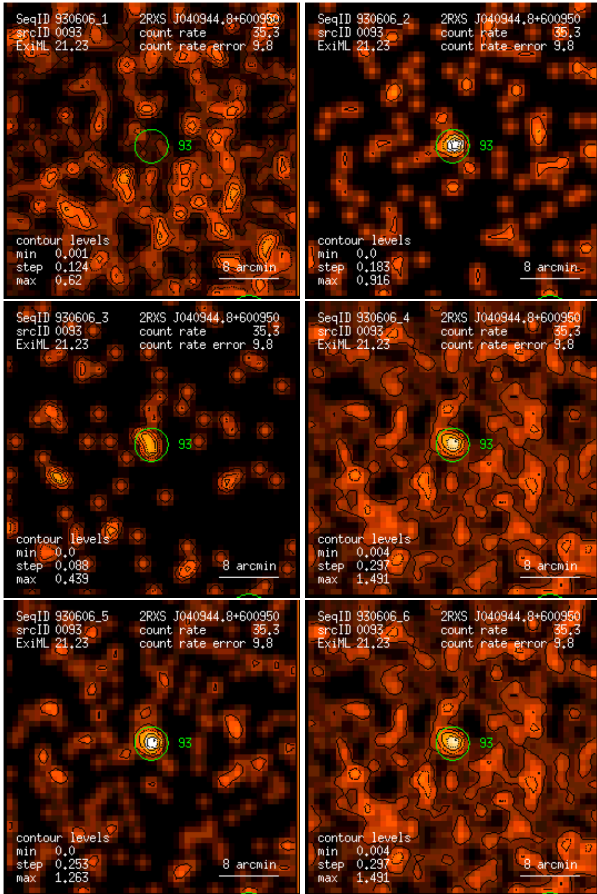
Figure 93: RASS 930606: detection 0093: band rate images, Gaussian filter: (1) PSPC channels 11 – 41, (2) 52 – 90, (3) 91 – 201, (4) 11 – 235, (5) 52 – 201, (6) 11 – 201. Broad band rates in counts/ks. Band rate contour levels in counts/ks/arcmin 2 .
