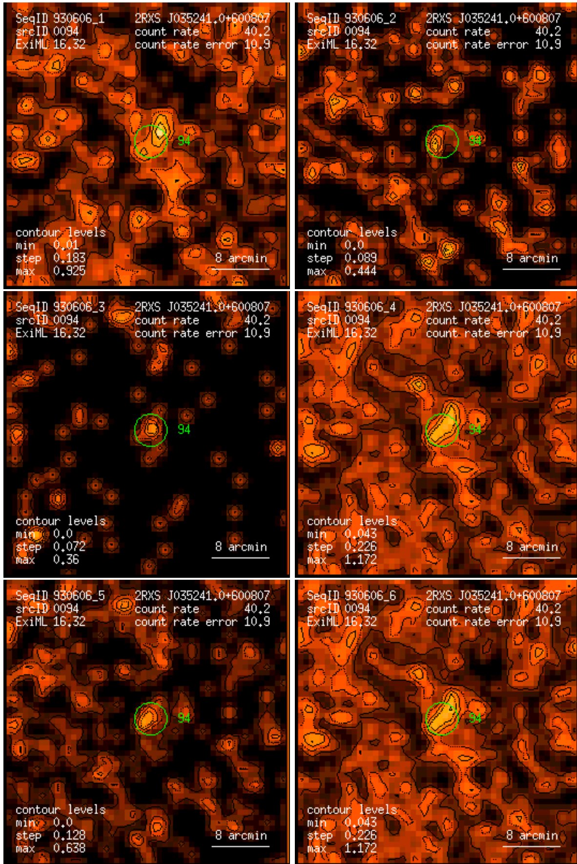
Figure 94: RASS 930606: detection 0094: band rate images, Gaussian filter: (1) PSPC channels 11 – 41, (2) 52 – 90, (3) 91 – 201, (4) 11 – 235, (5) 52 – 201, (6) 11 – 201. Broad band rates in counts/ks. Band rate contour levels in counts/ks/arcmin 2 .
