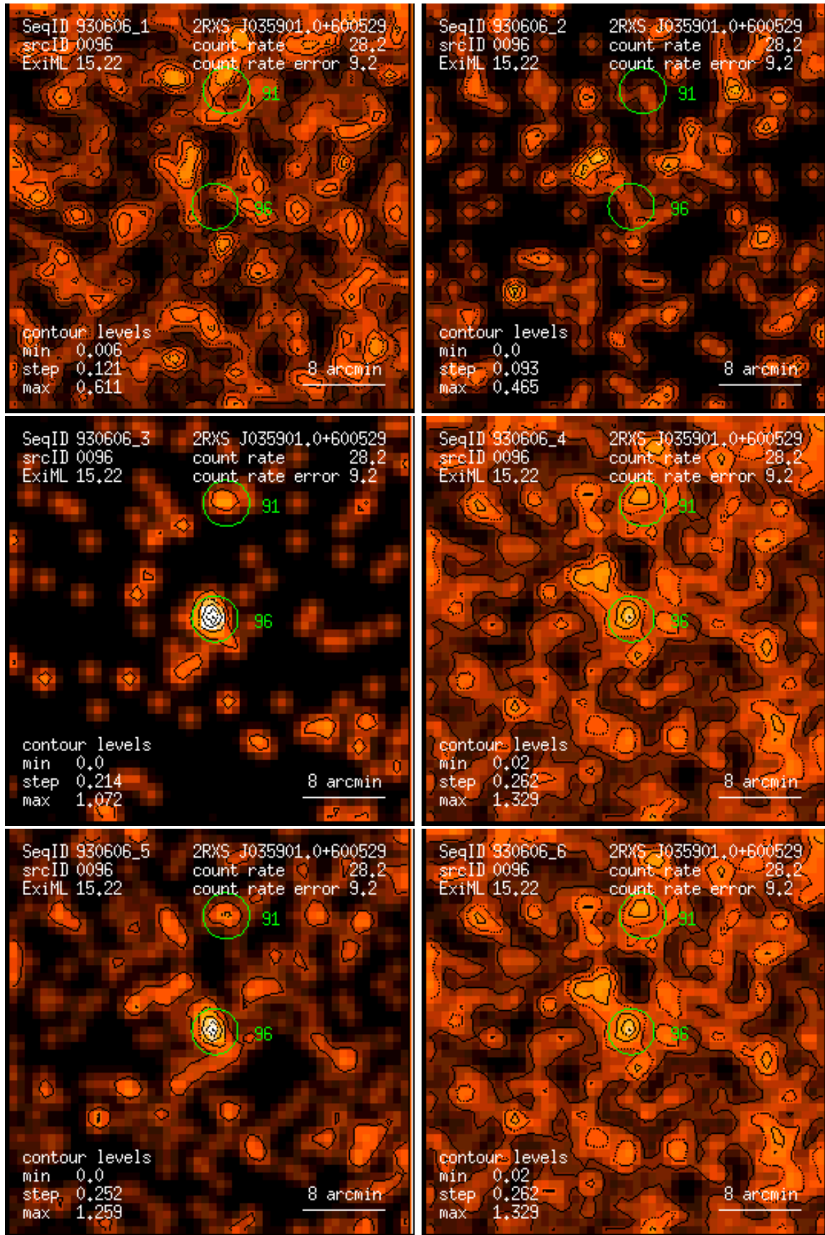
Figure 96: RASS 930606: detection 0096: band rate images, Gaussian filter: (1) PSPC channels 11 – 41, (2) 52 – 90, (3) 91 – 201, (4) 11 – 235, (5) 52 – 201, (6) 11 – 201. Broad band rates in counts/ks. Band rate contour levels in counts/ks/arcmin 2 .
