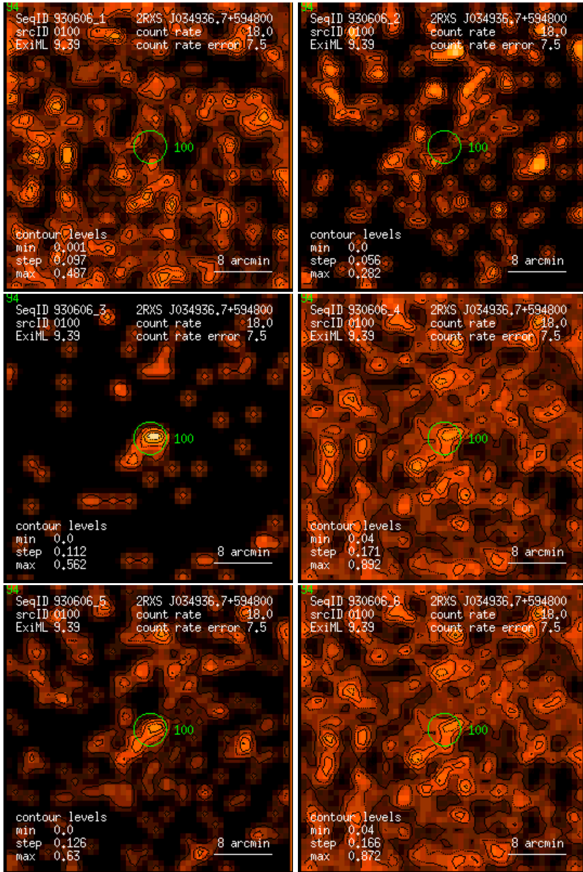
Figure 100: RASS 930606: detection 0100: band rate images, Gaussian filter: (1) PSPC channels 11 – 41, (2) 52 – 90, (3) 91 – 201, (4) 11 – 235, (5) 52 – 201, (6) 11 – 201. Broad band rates in counts/ks. Band rate contour levels in counts/ks/arcmin 2 .
