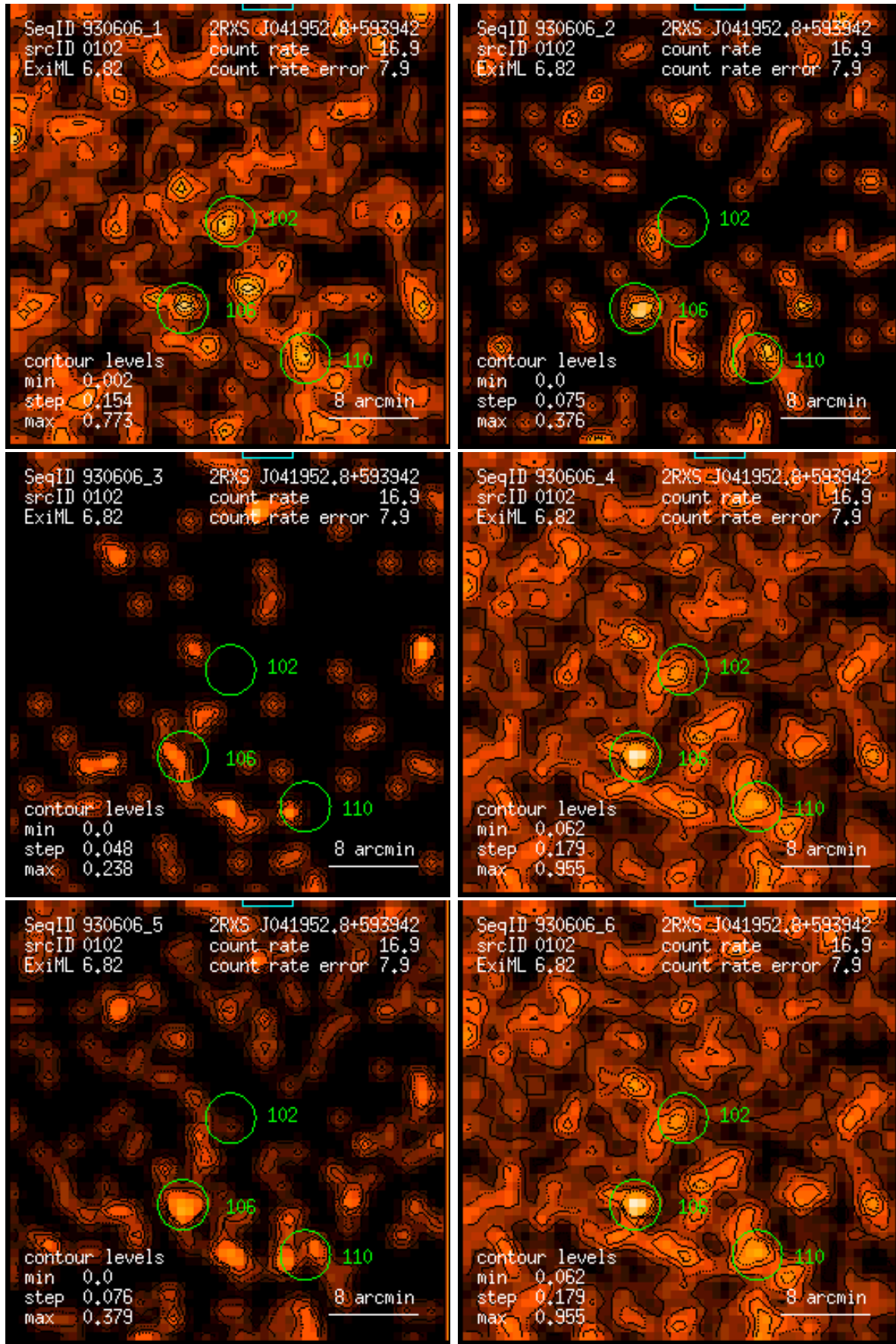
Figure 102: RASS 930606: detection 0102: band rate images, Gaussian filter: (1) PSPC channels 11 – 41, (2) 52 – 90, (3) 91 – 201, (4) 11 – 235, (5) 52 – 201, (6) 11 – 201. Broad band rates in counts/ks. Band rate contour levels in counts/ks/arcmin 2 .
