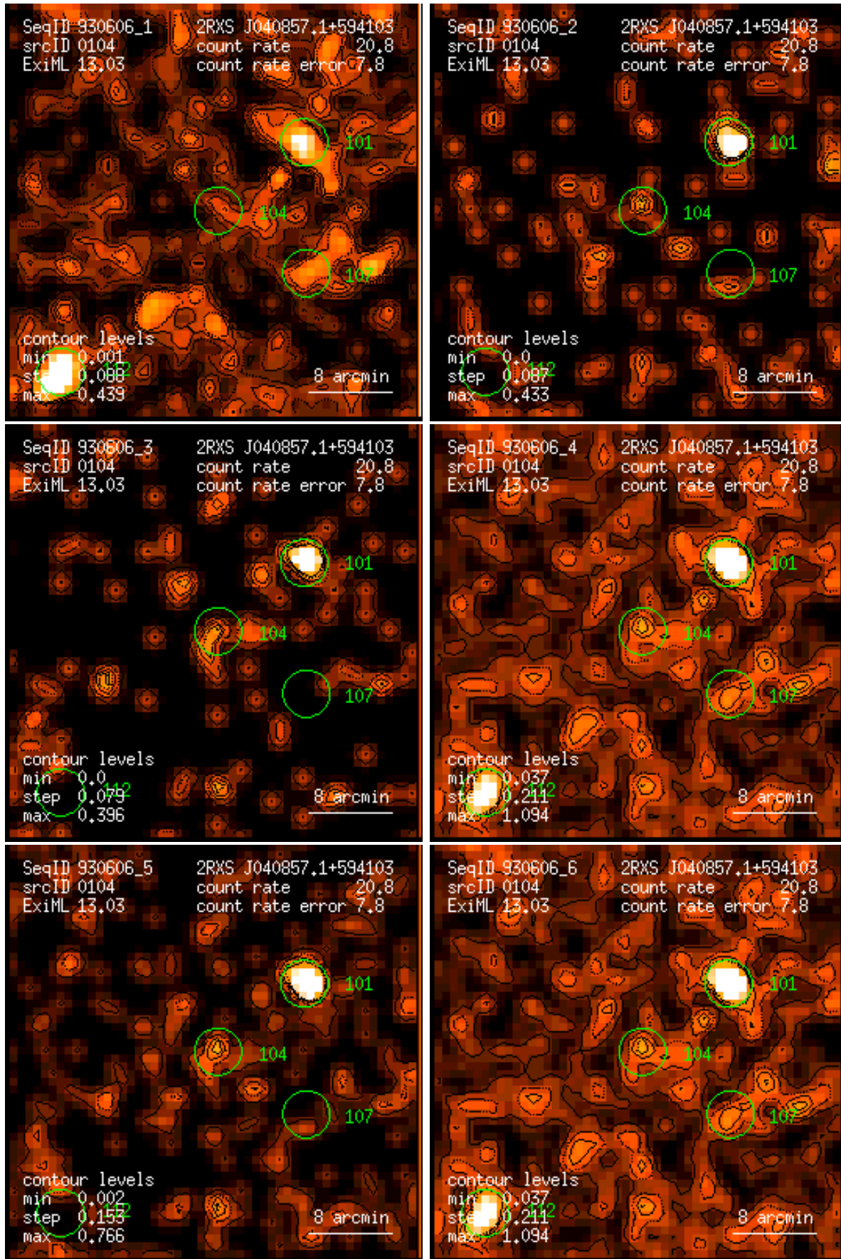
Figure 104: RASS 930606: detection 0104: band rate images, Gaussian filter: (1) PSPC channels 11 – 41, (2) 52 – 90, (3) 91 – 201, (4) 11 – 235, (5) 52 – 201, (6) 11 – 201. Broad band rates in counts/ks. Band rate contour levels in counts/ks/arcmin 2 .
