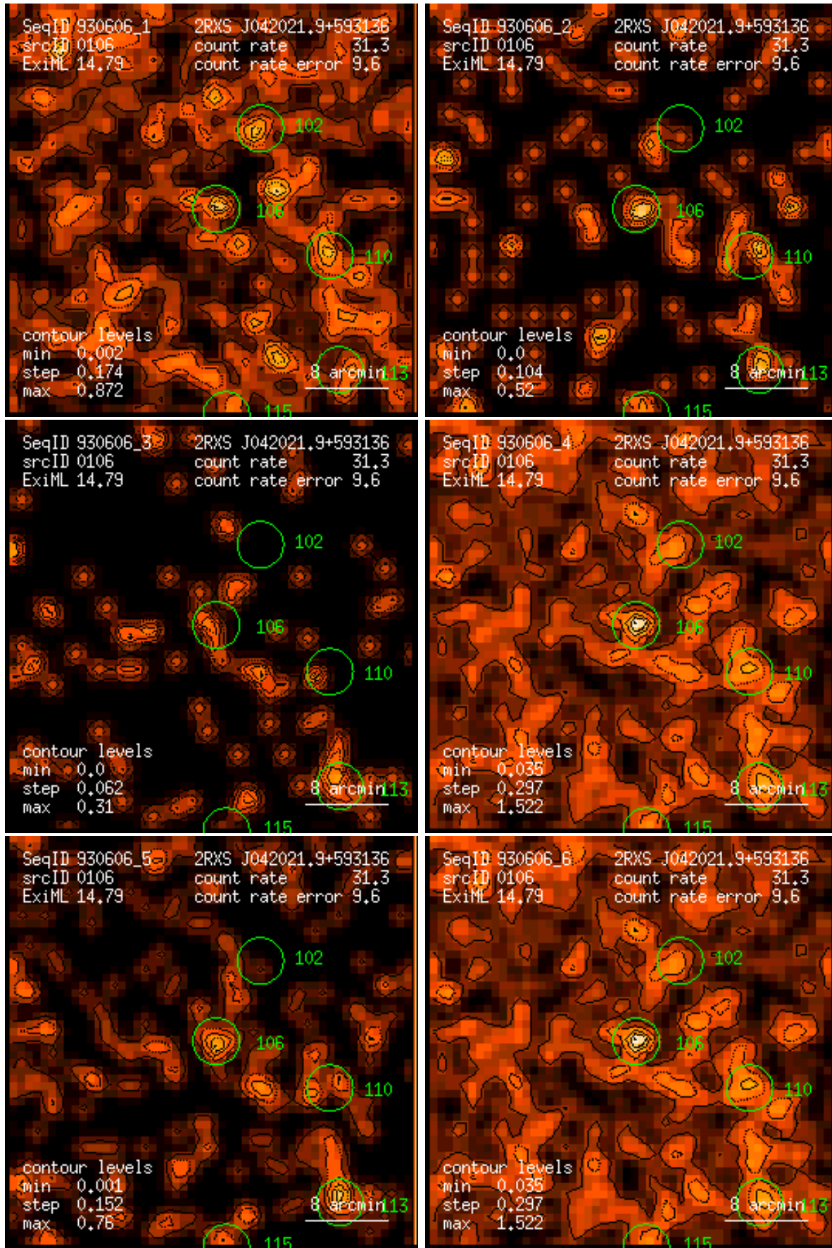
Figure 106: RASS 930606: detection 0106: band rate images, Gaussian filter: (1) PSPC channels 11 – 41, (2) 52 – 90, (3) 91 – 201, (4) 11 – 235, (5) 52 – 201, (6) 11 – 201. Broad band rates in counts/ks. Band rate contour levels in counts/ks/arcmin 2 .
