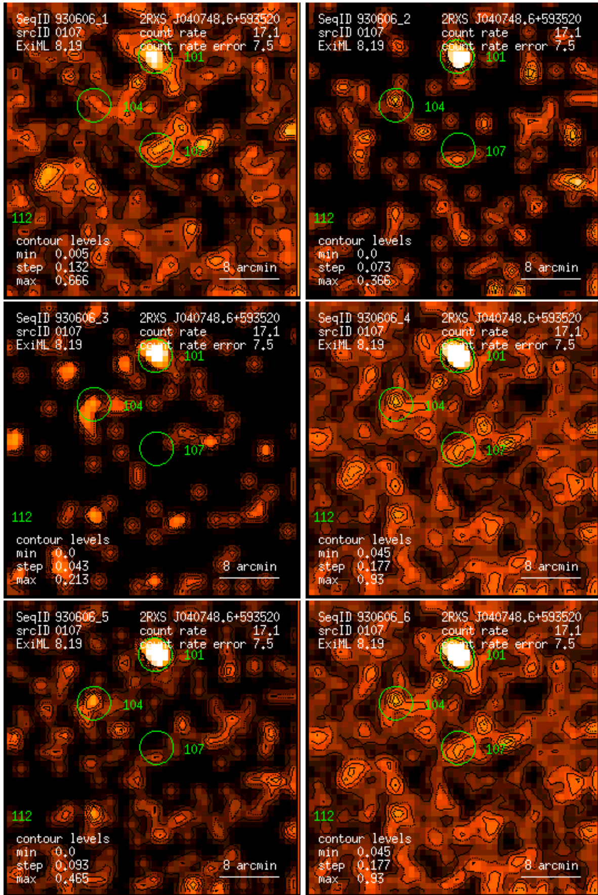
Figure 107: RASS 930606: detection 0107: band rate images, Gaussian filter: (1) PSPC channels 11 – 41, (2) 52 – 90, (3) 91 – 201, (4) 11 – 235, (5) 52 – 201, (6) 11 – 201. Broad band rates in counts/ks. Band rate contour levels in counts/ks/arcmin 2 .
