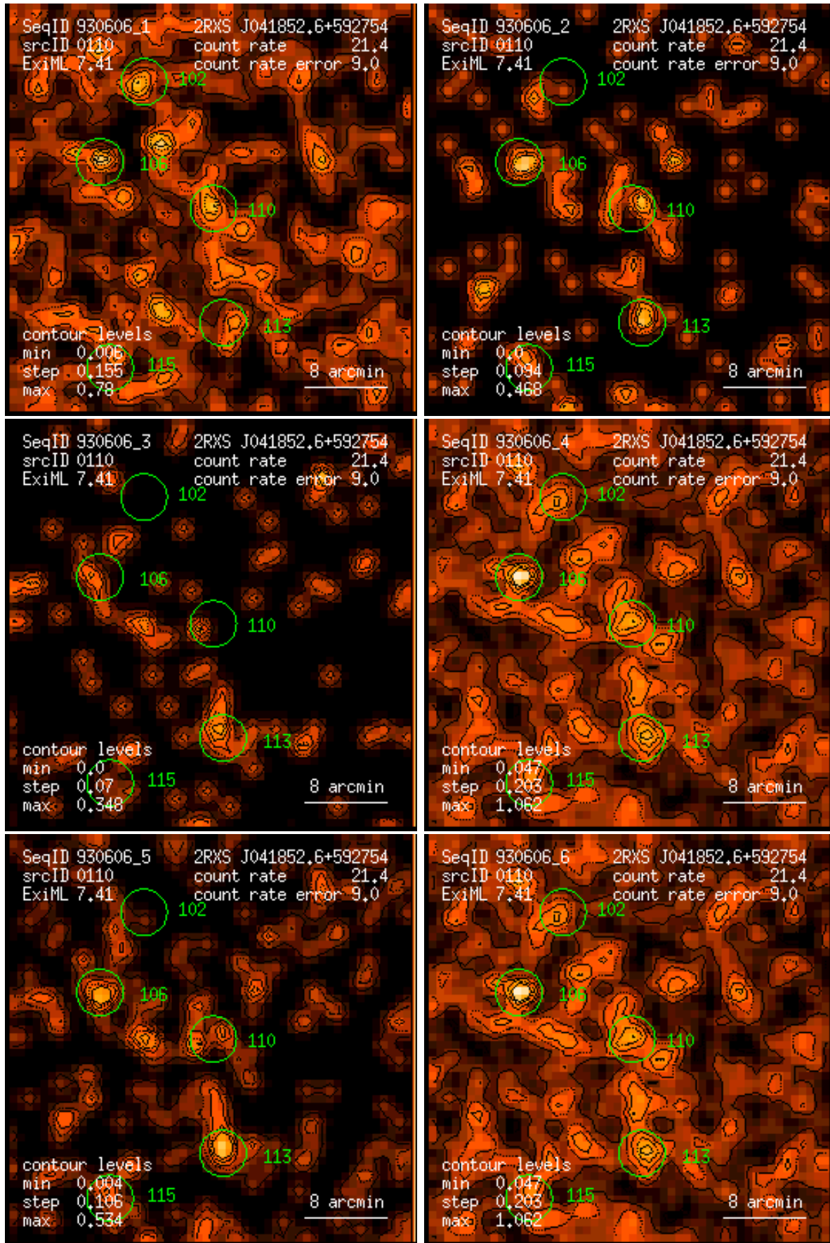
Figure 110: RASS 930606: detection 0110: band rate images, Gaussian filter: (1) PSPC channels 11 – 41, (2) 52 – 90, (3) 91 – 201, (4) 11 – 235, (5) 52 – 201, (6) 11 – 201. Broad band rates in counts/ks. Band rate contour levels in counts/ks/arcmin 2 .
