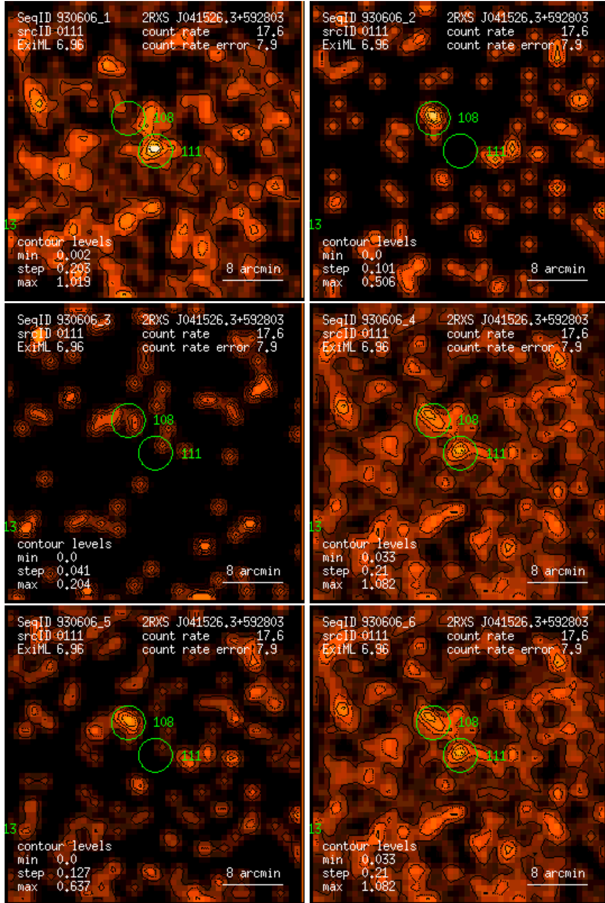
Figure 111: RASS 930606: detection 0111: band rate images, Gaussian filter: (1) PSPC channels 11 – 41, (2) 52 – 90, (3) 91 – 201, (4) 11 – 235, (5) 52 – 201, (6) 11 – 201. Broad band rates in counts/ks. Band rate contour levels in counts/ks/arcmin 2 .
