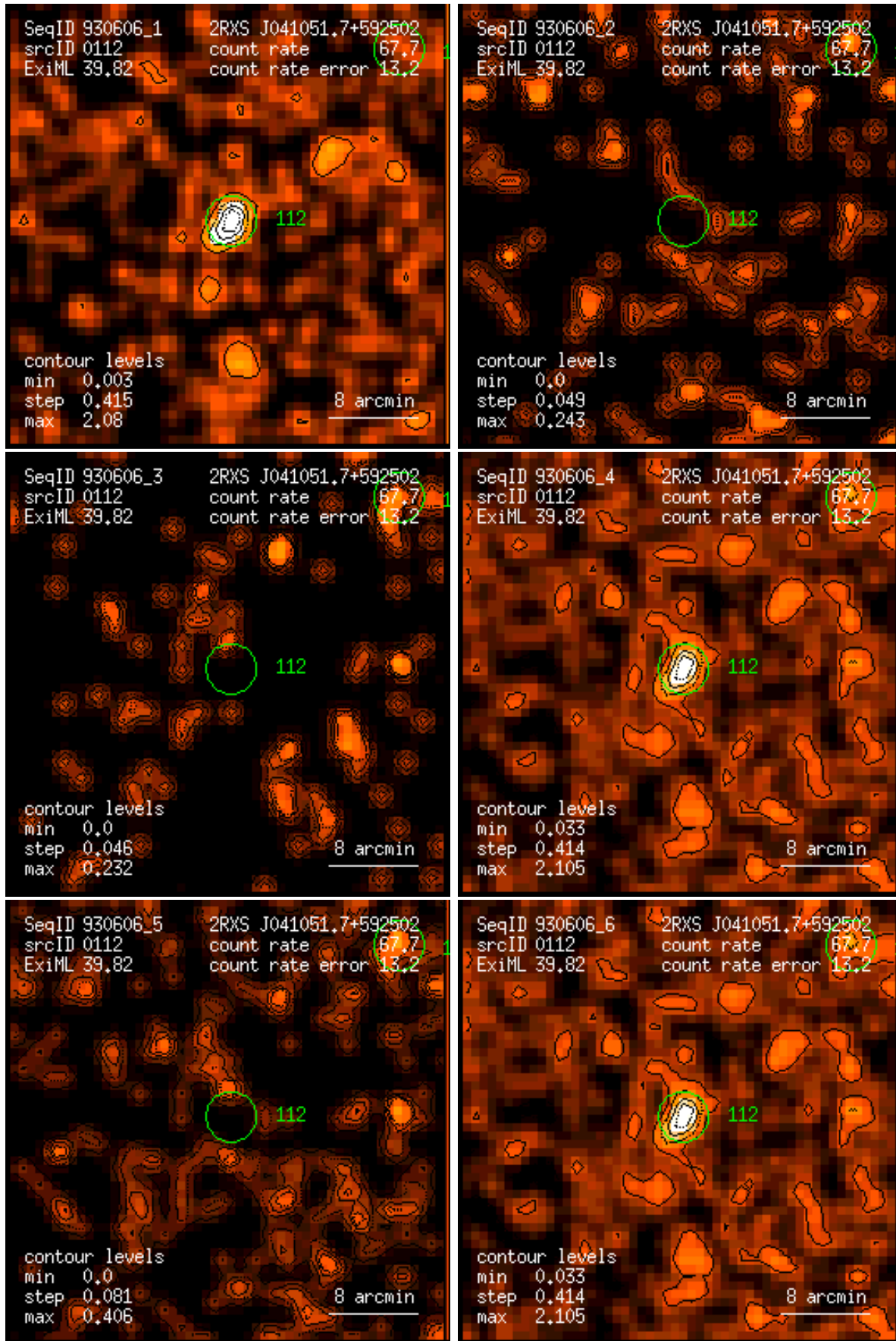
Figure 112: RASS 930606: detection 0112: band rate images, Gaussian filter: (1) PSPC channels 11 – 41, (2) 52 – 90, (3) 91 – 201, (4) 11 – 235, (5) 52 – 201, (6) 11 – 201. Broad band rates in counts/ks. Band rate contour levels in counts/ks/arcmin 2 .
