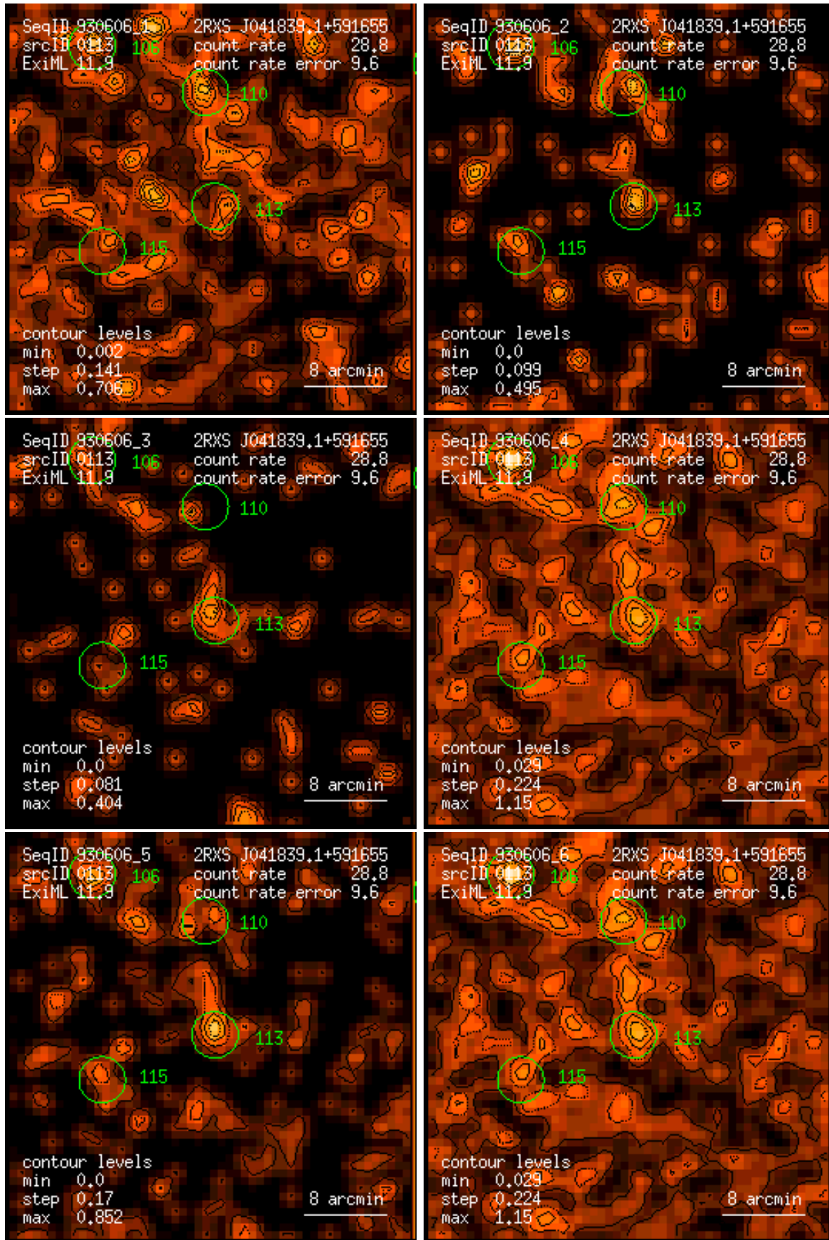
Figure 113: RASS 930606: detection 0113: band rate images, Gaussian filter: (1) PSPC channels 11 – 41, (2) 52 – 90, (3) 91 – 201, (4) 11 – 235, (5) 52 – 201, (6) 11 – 201. Broad band rates in counts/ks. Band rate contour levels in counts/ks/arcmin 2 .
