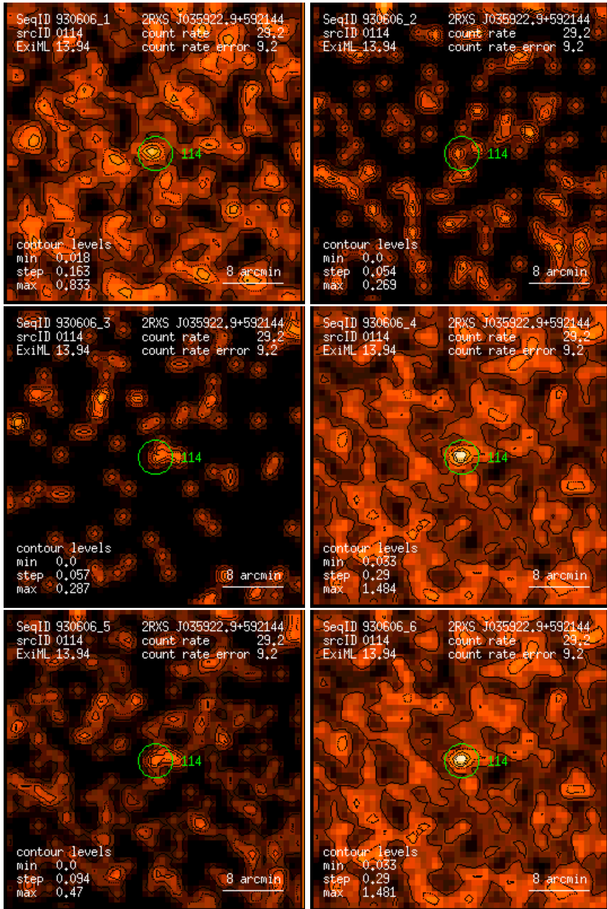
Figure 114: RASS 930606: detection 0114: band rate images, Gaussian filter: (1) PSPC channels 11 – 41, (2) 52 – 90, (3) 91 – 201, (4) 11 – 235, (5) 52 – 201, (6) 11 – 201. Broad band rates in counts/ks. Band rate contour levels in counts/ks/arcmin 2 .
