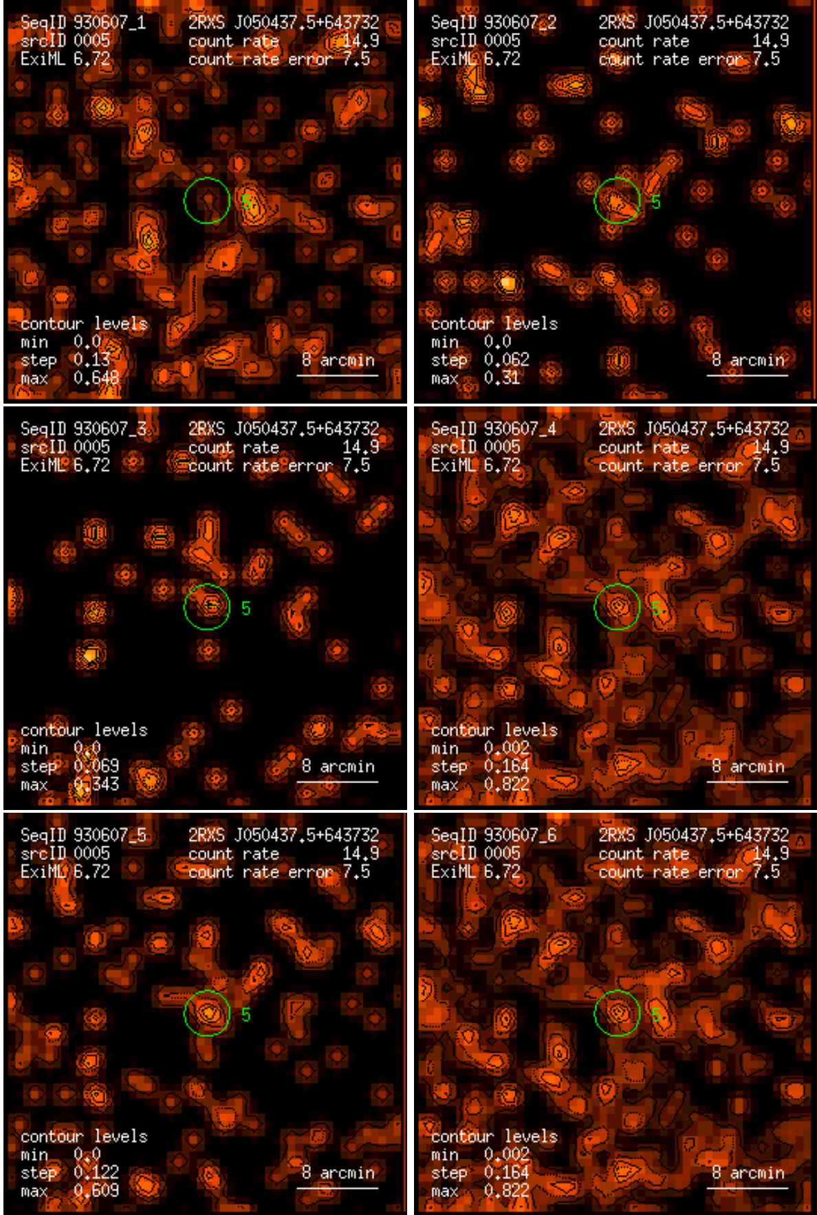
Figure 5: RASS 930607: detection 0005: band rate images, Gaussian filter: (1) PSPC channels 11 – 41, (2) 52 – 90, (3) 91 – 201, (4) 11 – 235, (5) 52 – 201, (6) 11 – 201. Broad band rates in counts/ks. Band rate contour levels in counts/ks/arcmin 2 .
