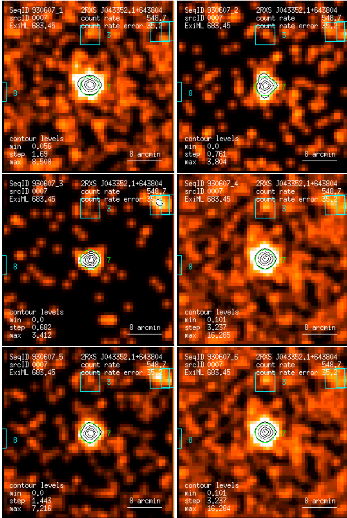
Figure 7: RASS 930607: detection 0007: band rate images, Gaussian filter: (1) PSPC channels 11 – 41, (2) 52 – 90, (3) 91 – 201, (4) 11 – 235, (5) 52 – 201, (6) 11 – 201. Broad band rates in counts/ks. Band rate contour levels in counts/ks/arcmin 2 .
