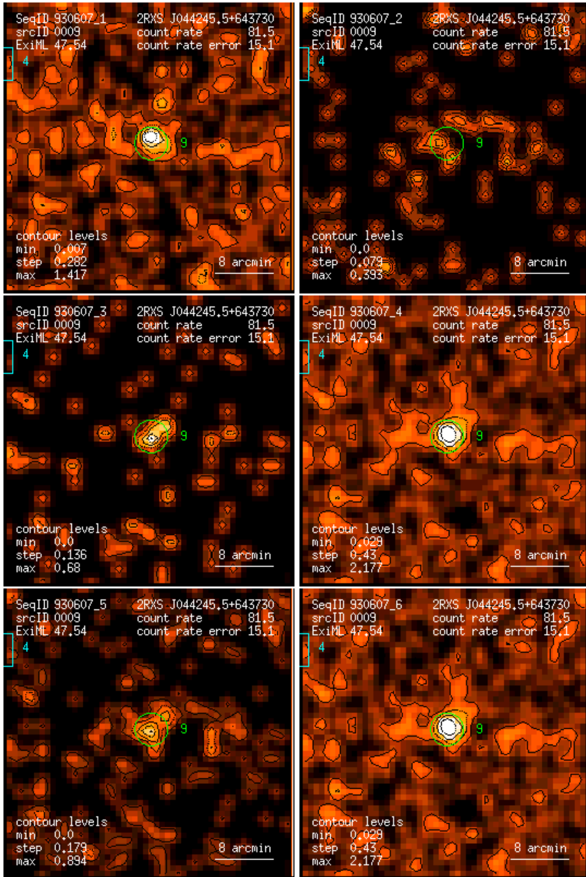
Figure 9: RASS 930607: detection 0009: band rate images, Gaussian filter: (1) PSPC channels 11 – 41, (2) 52 – 90, (3) 91 – 201, (4) 11 – 235, (5) 52 – 201, (6) 11 – 201. Broad band rates in counts/ks. Band rate contour levels in counts/ks/arcmin 2 .
