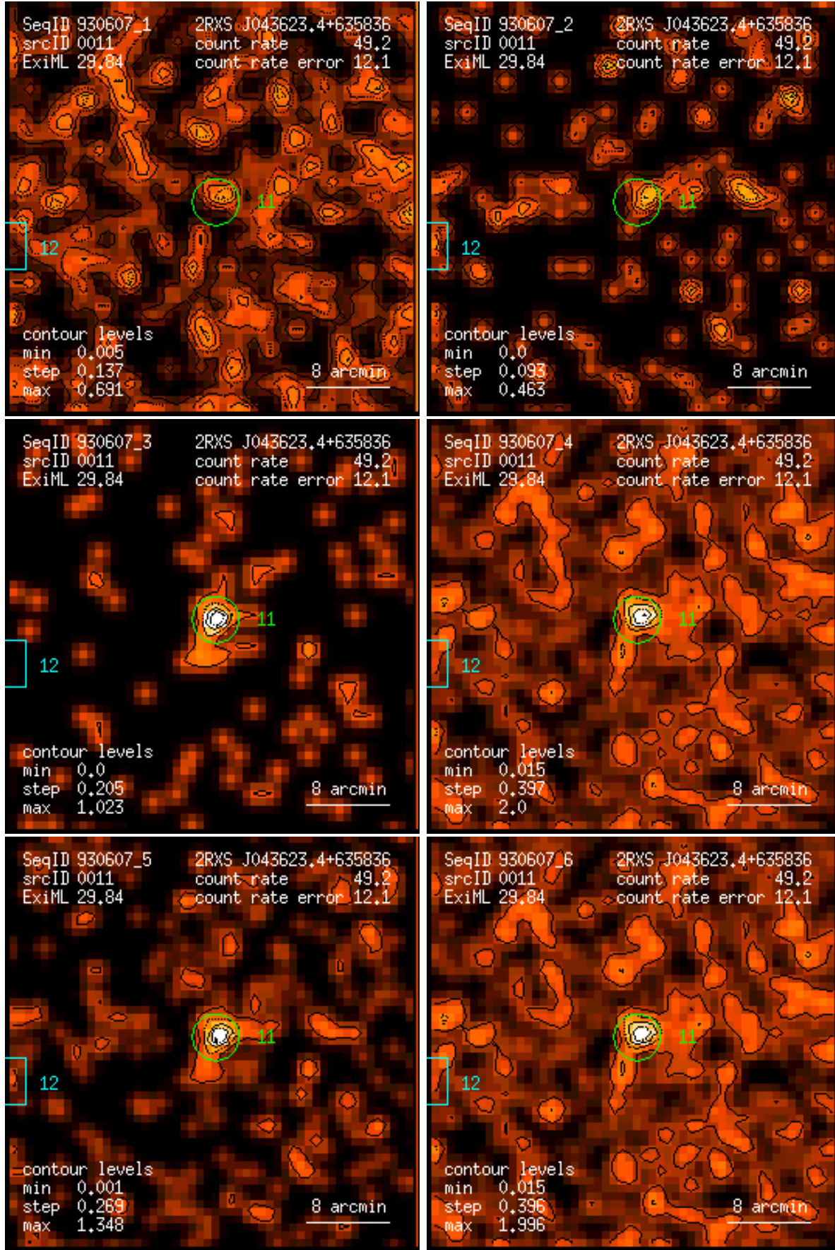
Figure 11: RASS 930607: detection 0011: band rate images, Gaussian filter: (1) PSPC channels 11 – 41, (2) 52 – 90, (3) 91 – 201, (4) 11 – 235, (5) 52 – 201, (6) 11 – 201. Broad band rates in counts/ks. Band rate contour levels in counts/ks/arcmin 2 .
