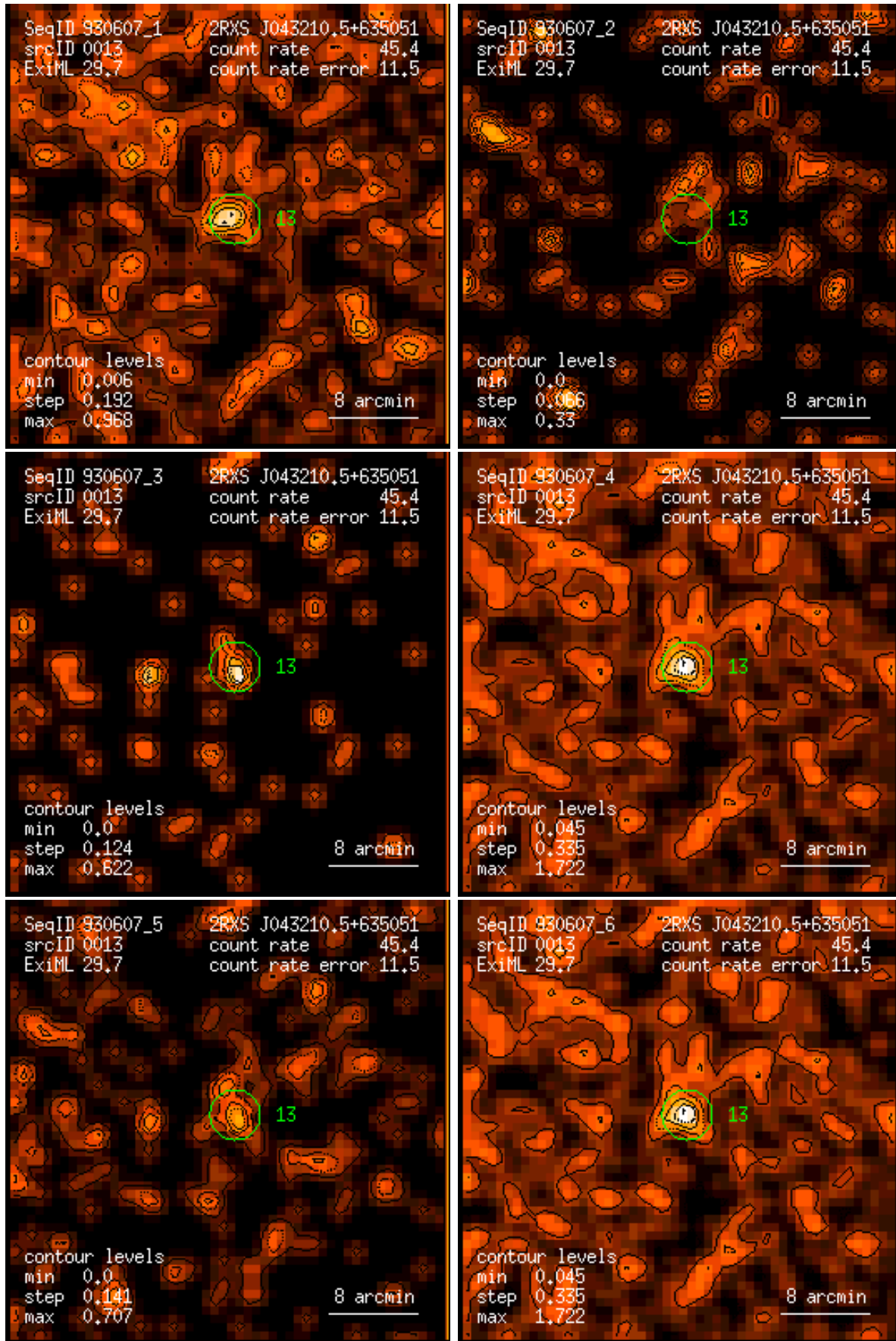
Figure 13: RASS 930607: detection 0013: band rate images, Gaussian filter: (1) PSPC channels 11 – 41, (2) 52 – 90, (3) 91 – 201, (4) 11 – 235, (5) 52 – 201, (6) 11 – 201. Broad band rates in counts/ks. Band rate contour levels in counts/ks/arcmin 2 .
