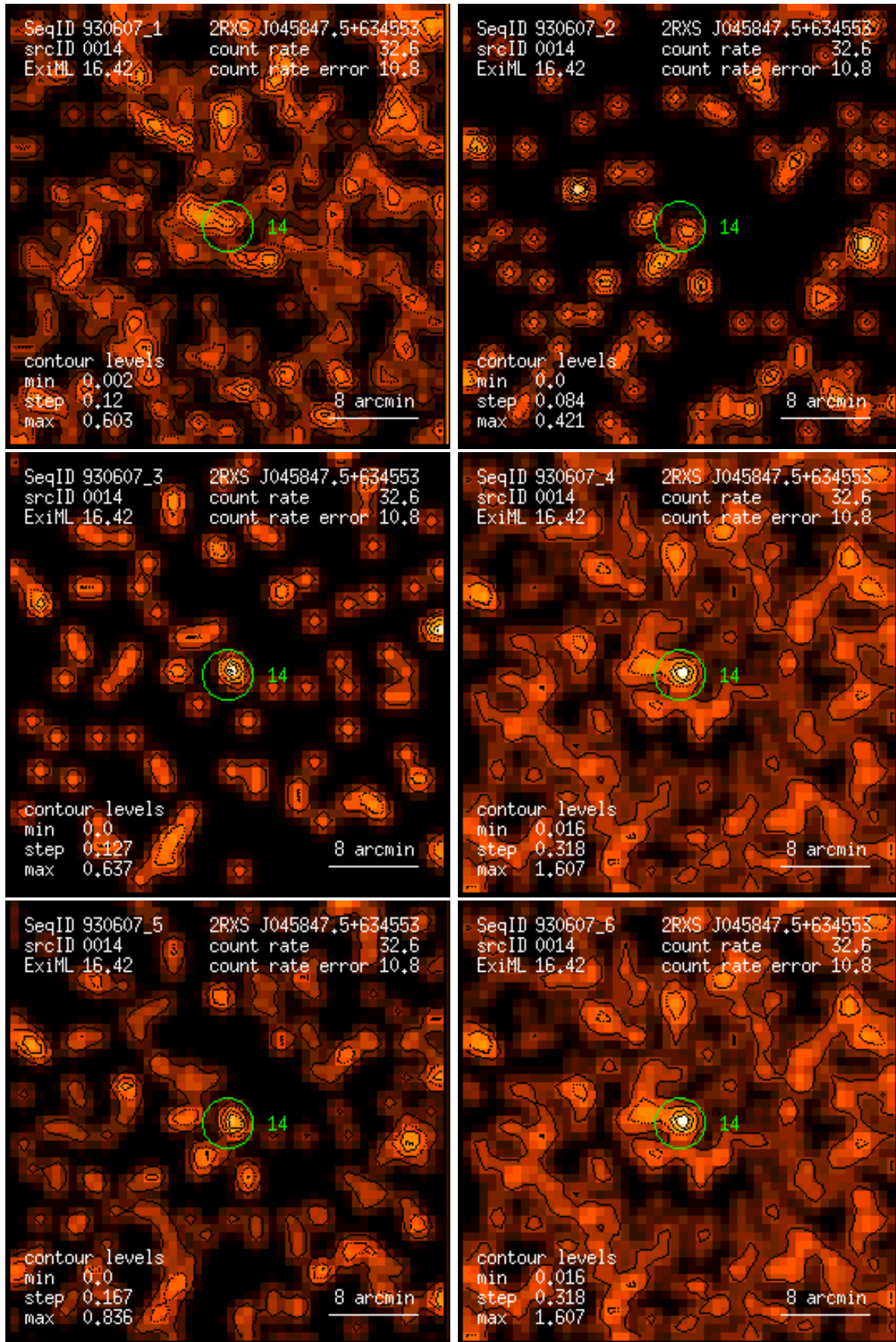
Figure 14: RASS 930607: detection 0014: band rate images, Gaussian filter: (1) PSPC channels 11 – 41, (2) 52 – 90, (3) 91 – 201, (4) 11 – 235, (5) 52 – 201, (6) 11 – 201. Broad band rates in counts/ks. Band rate contour levels in counts/ks/arcmin 2 .
