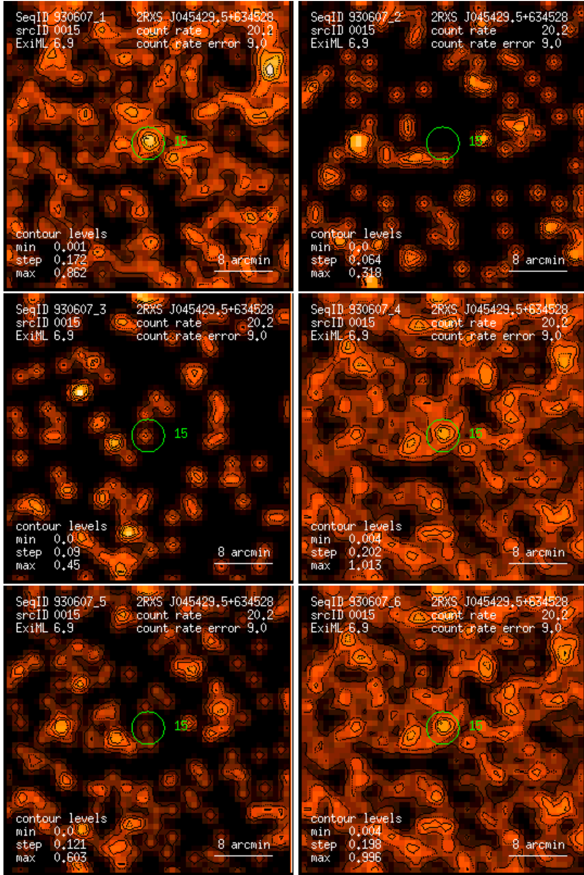
Figure 15: RASS 930607: detection 0015: band rate images, Gaussian filter: (1) PSPC channels 11 – 41, (2) 52 – 90, (3) 91 – 201, (4) 11 – 235, (5) 52 – 201, (6) 11 – 201. Broad band rates in counts/ks. Band rate contour levels in counts/ks/arcmin 2 .
