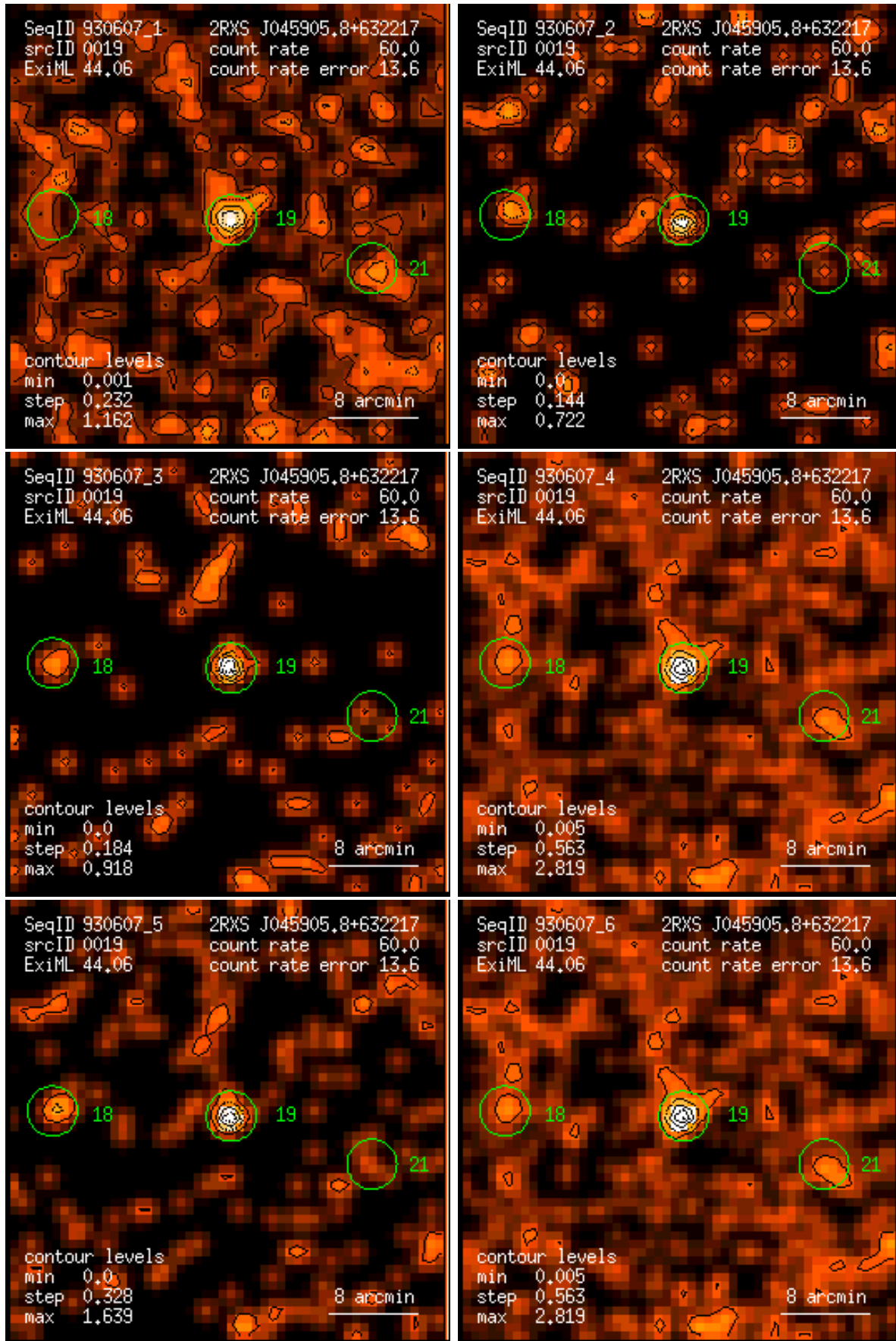
Figure 19: RASS 930607: detection 0019: band rate images, Gaussian filter: (1) PSPC channels 11 – 41, (2) 52 – 90, (3) 91 – 201, (4) 11 – 235, (5) 52 – 201, (6) 11 – 201. Broad band rates in counts/ks. Band rate contour levels in counts/ks/arcmin 2 .
