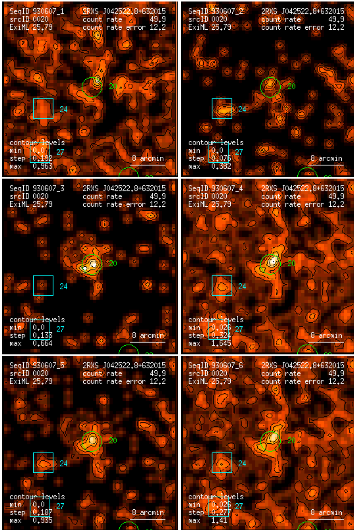
Figure 20: RASS 930607: detection 0020: band rate images, Gaussian filter: (1) PSPC channels 11 – 41, (2) 52 – 90, (3) 91 – 201, (4) 11 – 235, (5) 52 – 201, (6) 11 – 201. Broad band rates in counts/ks. Band rate contour levels in counts/ks/arcmin 2 .
