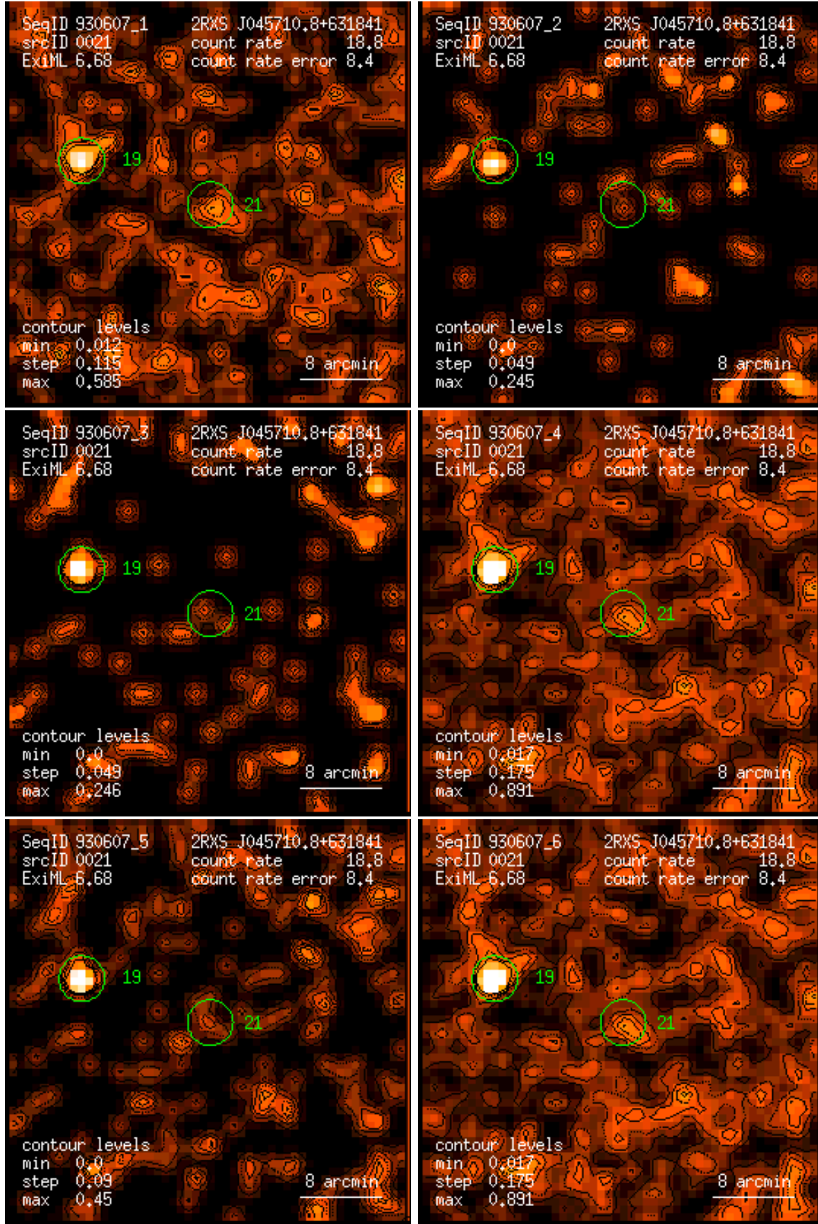
Figure 21: RASS 930607: detection 0021: band rate images, Gaussian filter: (1) PSPC channels 11 – 41, (2) 52 – 90, (3) 91 – 201, (4) 11 – 235, (5) 52 – 201, (6) 11 – 201. Broad band rates in counts/ks. Band rate contour levels in counts/ks/arcmin 2 .
