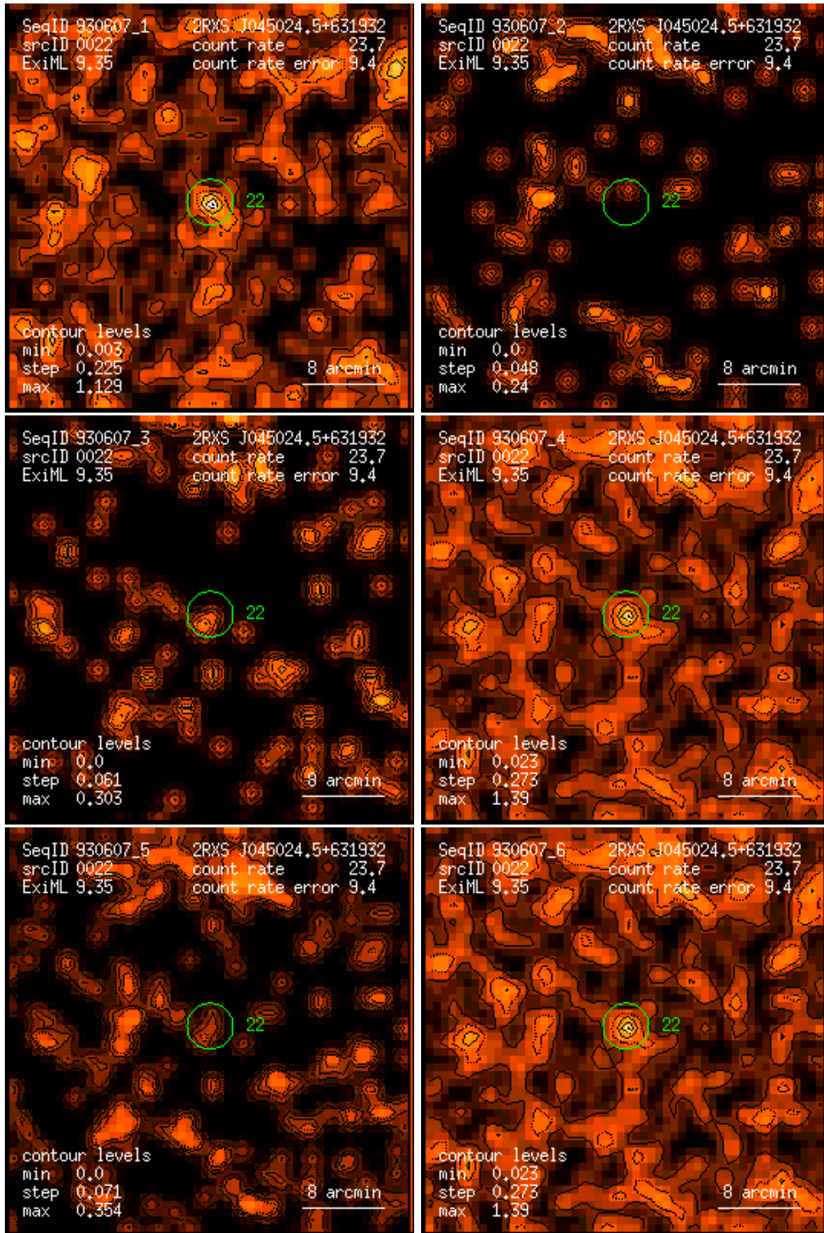
Figure 22: RASS 930607: detection 0022: band rate images, Gaussian filter: (1) PSPC channels 11 – 41, (2) 52 – 90, (3) 91 – 201, (4) 11 – 235, (5) 52 – 201, (6) 11 – 201. Broad band rates in counts/ks. Band rate contour levels in counts/ks/arcmin 2 .
