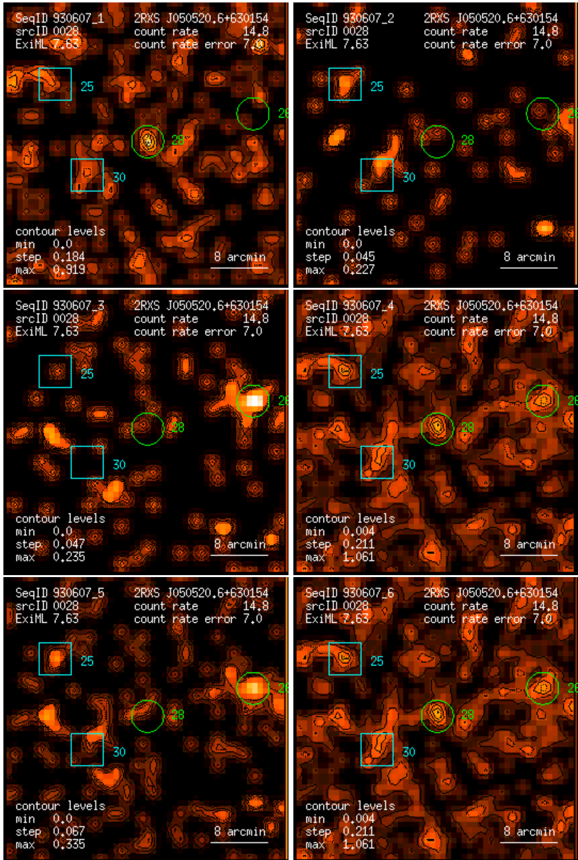
Figure 28: RASS 930607: detection 0028: band rate images, Gaussian filter: (1) PSPC channels 11 – 41, (2) 52 – 90, (3) 91 – 201, (4) 11 – 235, (5) 52 – 201, (6) 11 – 201. Broad band rates in counts/ks. Band rate contour levels in counts/ks/arcmin 2 .
