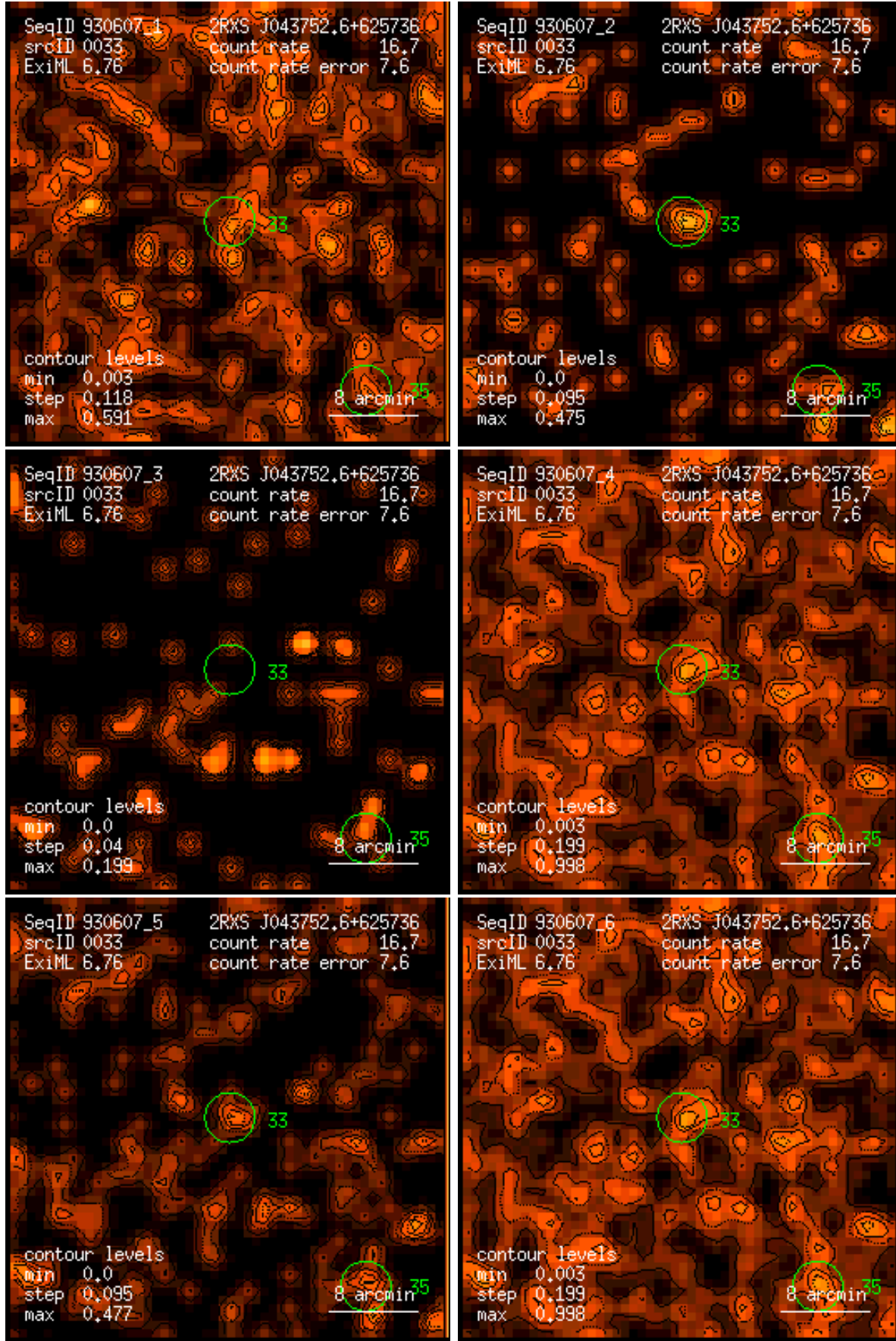
Figure 33: RASS 930607: detection 0033: band rate images, Gaussian filter: (1) PSPC channels 11 – 41, (2) 52 – 90, (3) 91 – 201, (4) 11 – 235, (5) 52 – 201, (6) 11 – 201. Broad band rates in counts/ks. Band rate contour levels in counts/ks/arcmin 2 .
