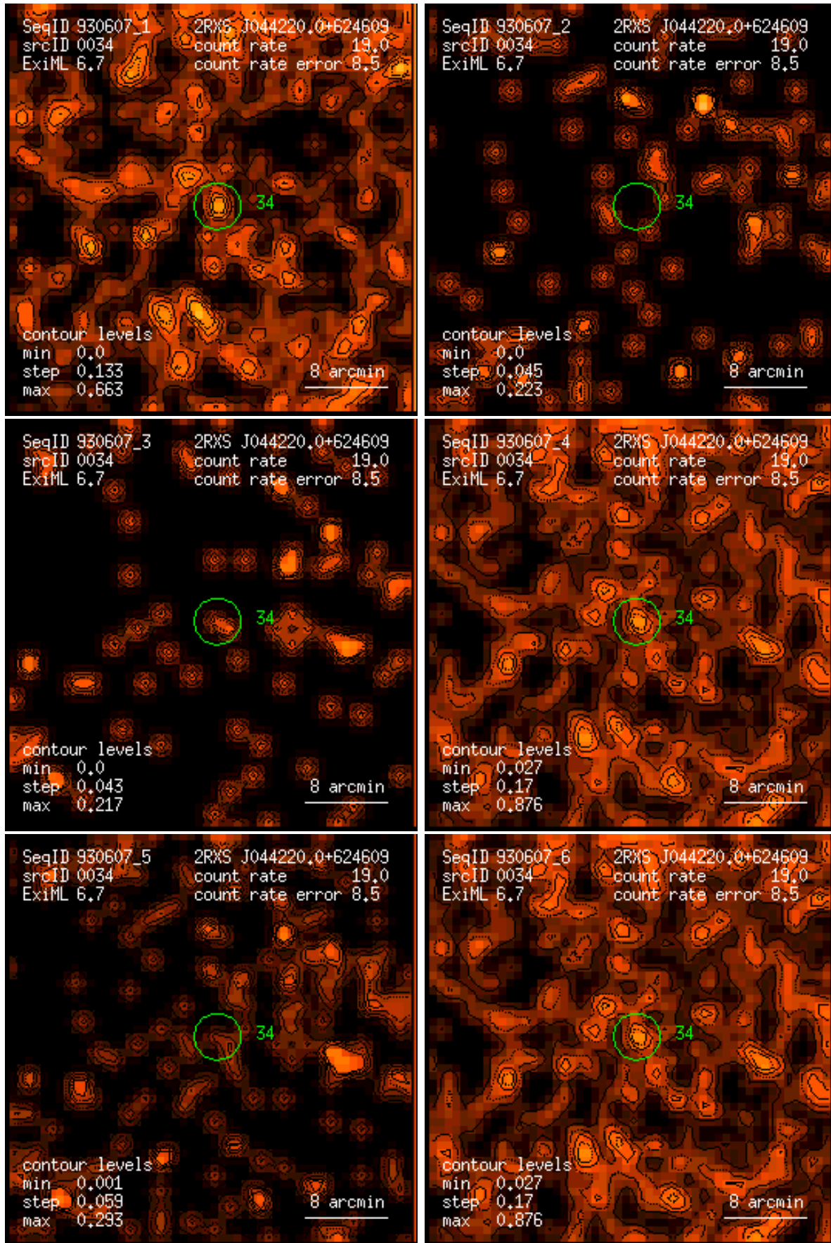
Figure 34: RASS 930607: detection 0034: band rate images, Gaussian filter: (1) PSPC channels 11 – 41, (2) 52 – 90, (3) 91 – 201, (4) 11 – 235, (5) 52 – 201, (6) 11 – 201. Broad band rates in counts/ks. Band rate contour levels in counts/ks/arcmin 2 .
